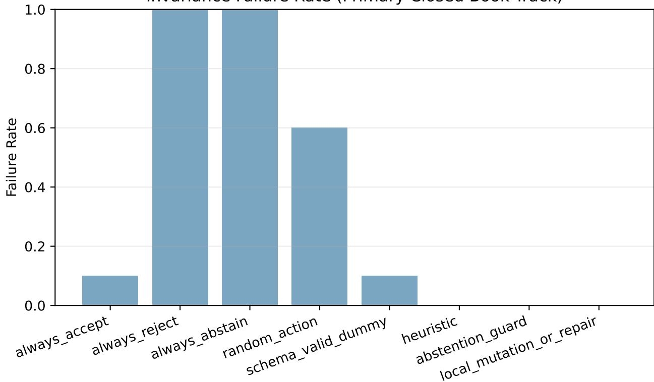
Invariance Failure Rate (Primary Closed Book Track)
