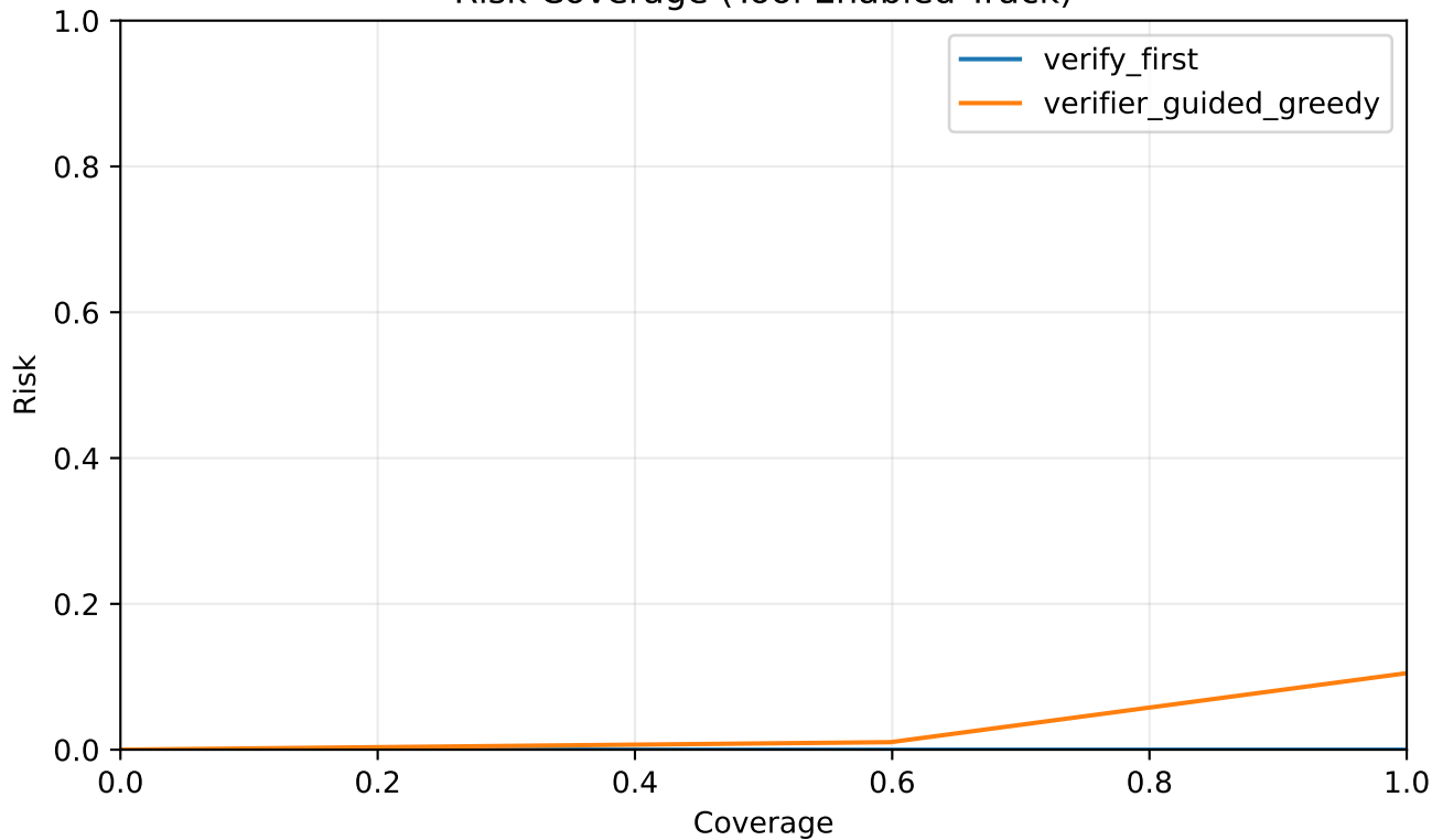
Risk-Coverage (Tool Enabled Track)
