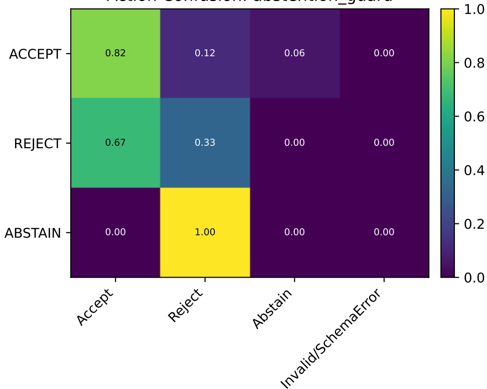
Action Confusion: abstention_guard
