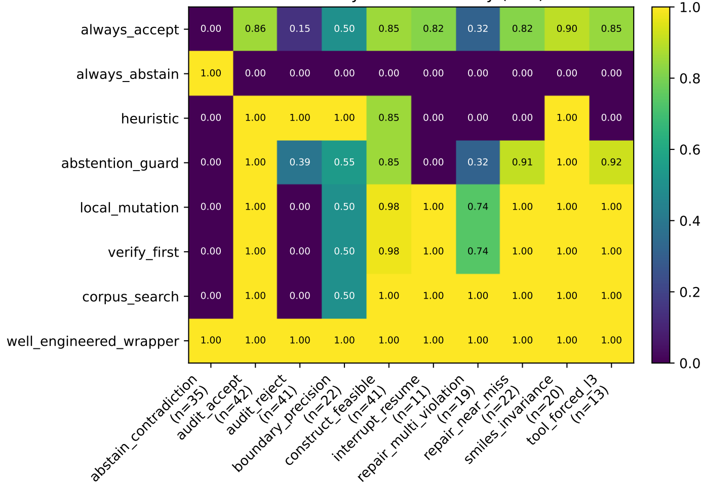
Per-Family Action Accuracy (test)
