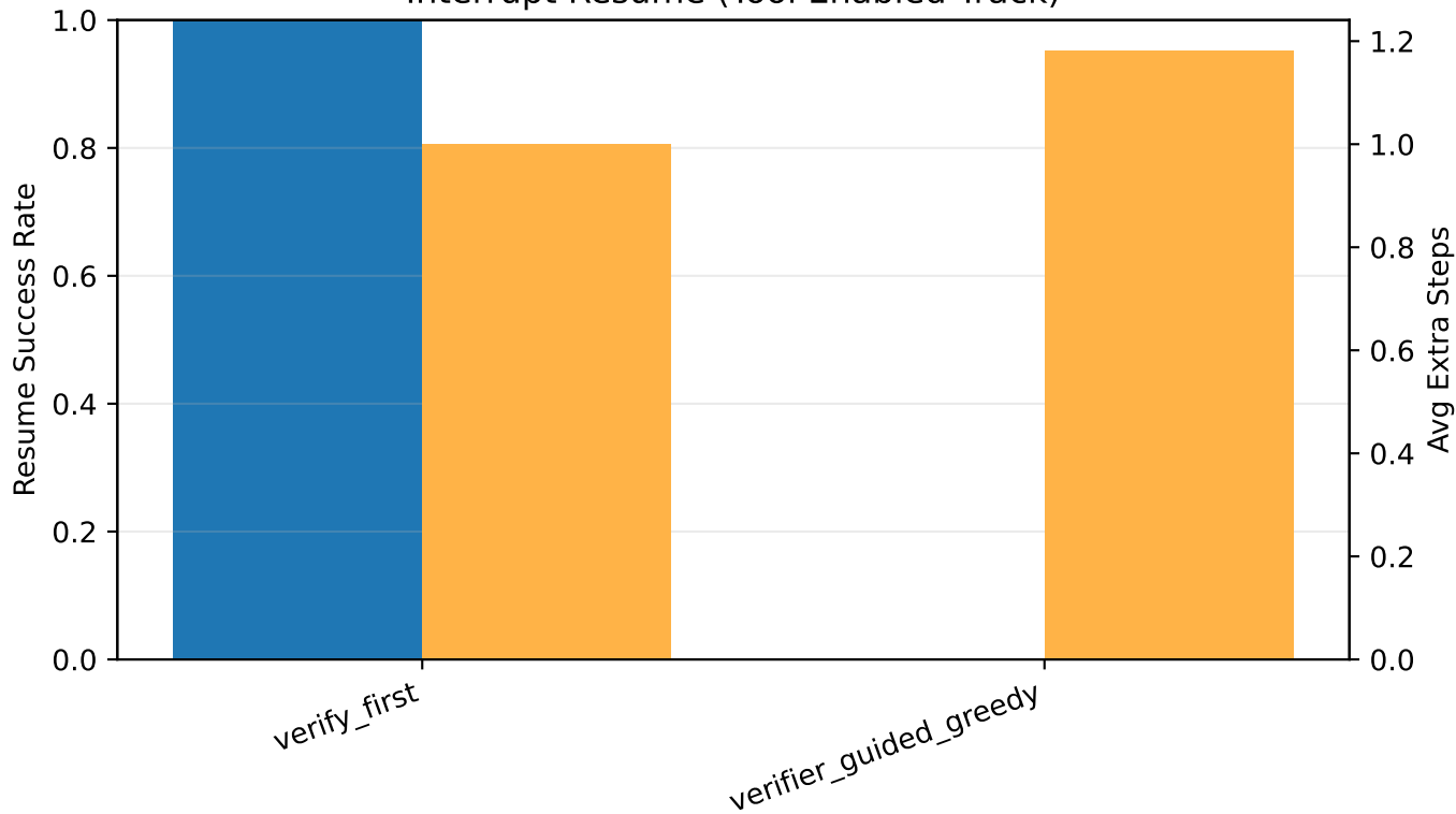
Interrupt Resume (Tool Enabled Track)
