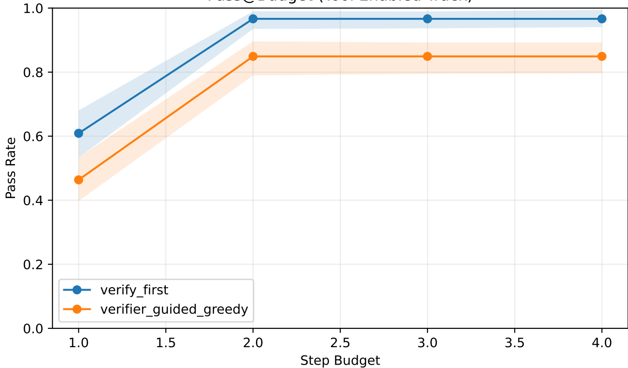
Pass@Budget (Tool Enabled Track)
