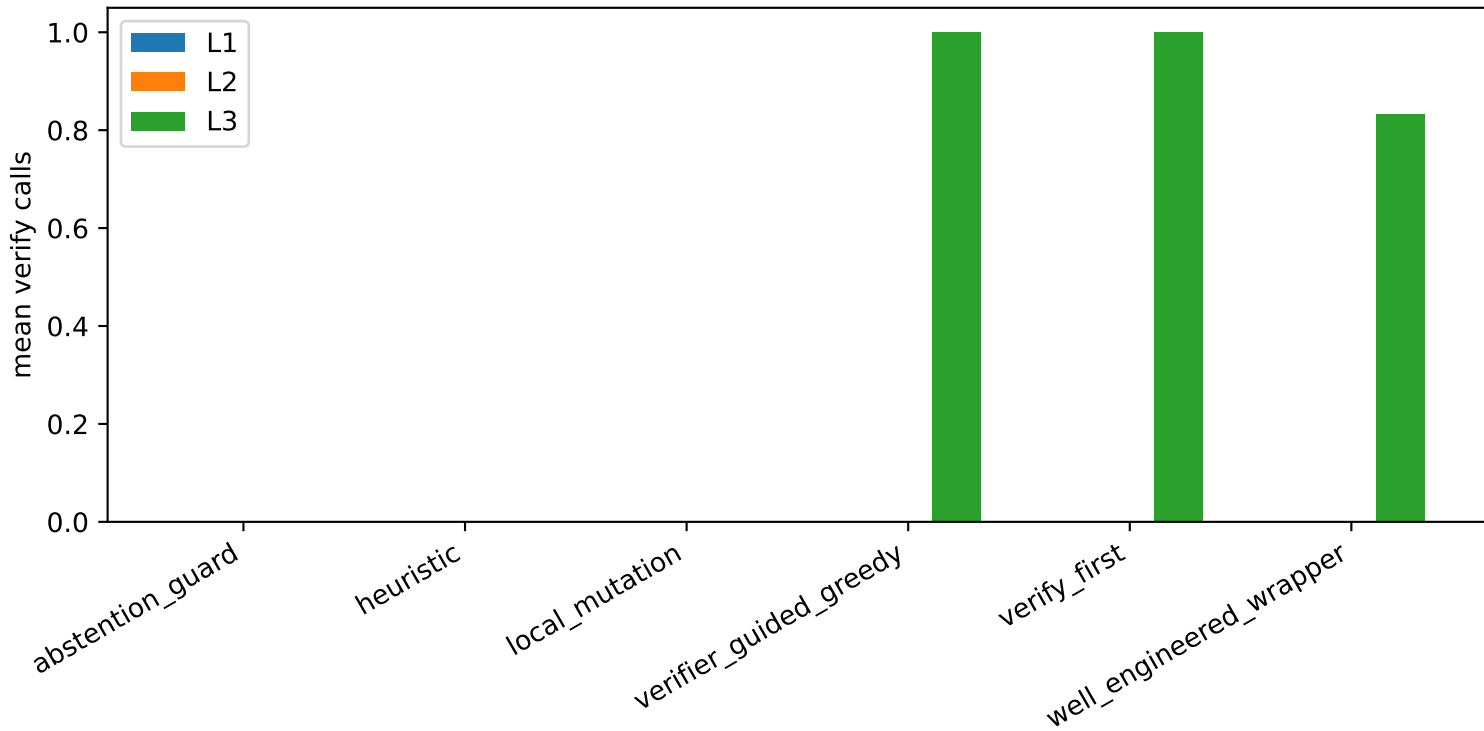
Mean Verify Calls by Native Protocol
