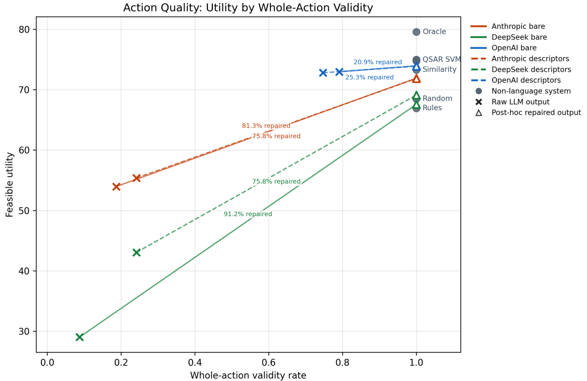
Figure 2: Action utility versus whole-action validity. Crosses are raw LLM outputs; open triangles are deterministic post-hoc-repaired outputs from the same responses. Connecting lines show harness intervention, not an additional model call; repaired points must not be interpreted as model-only performance.
