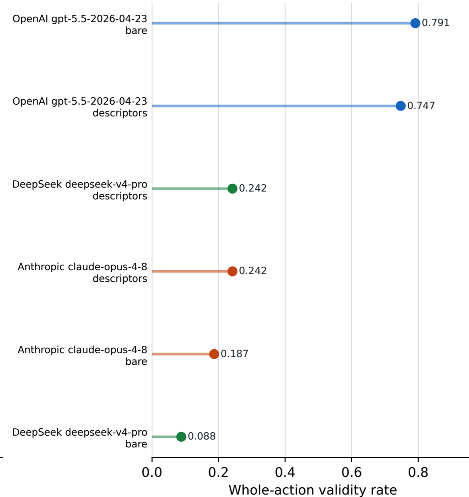
C. Raw LLM action validity
