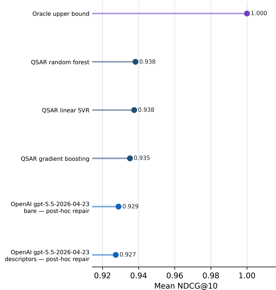
B. Leading NDCG@10
