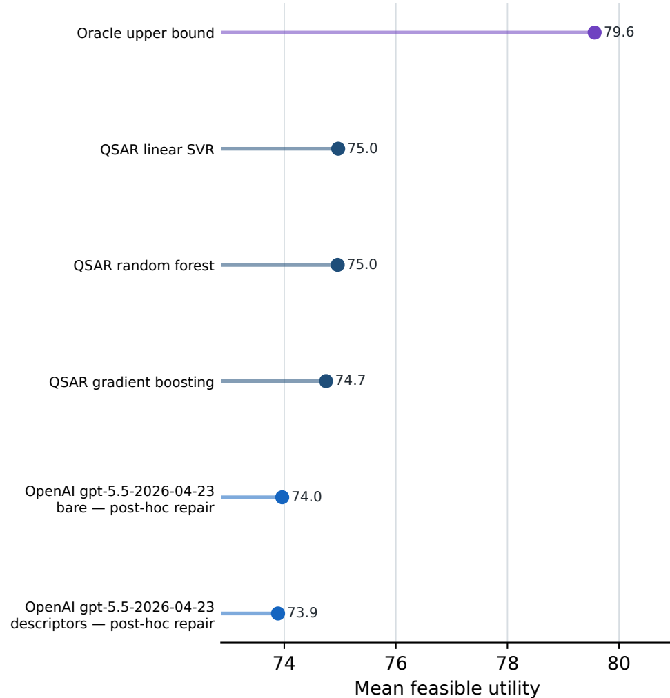
A. Leading feasible utility
