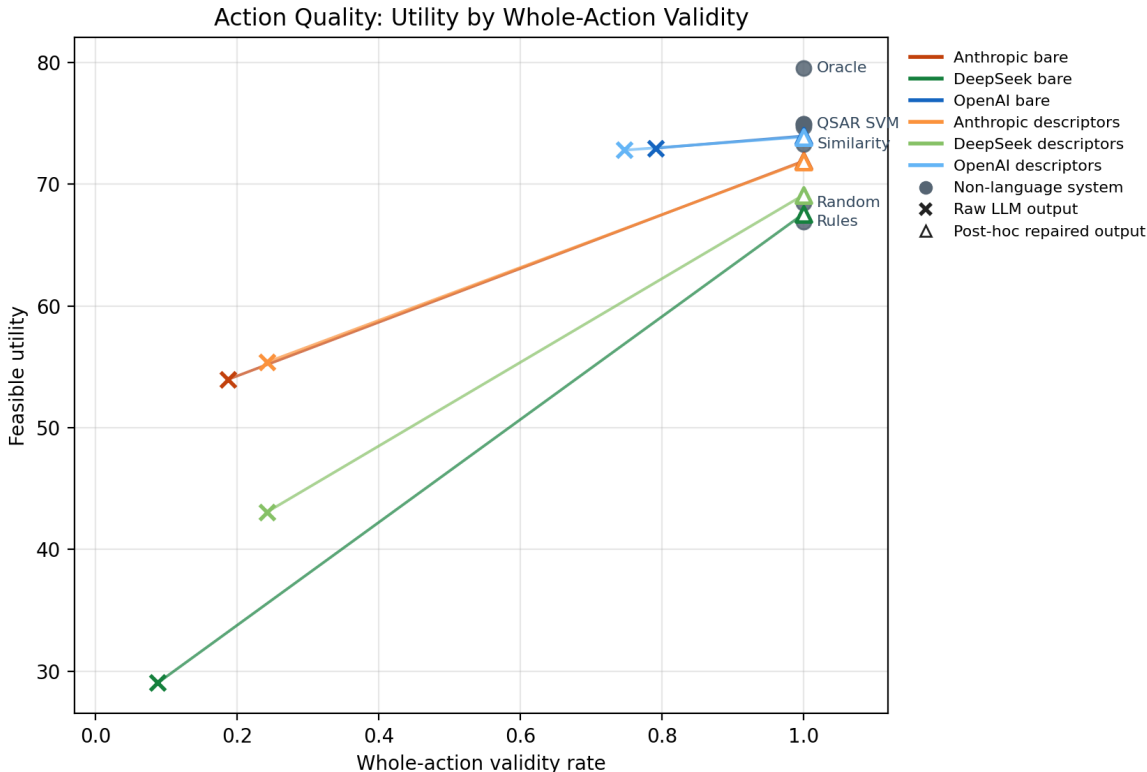
Figure 2: Action utility versus whole-action validity. Crosses are raw LLM outputs; open triangles are deterministic post-hoc-repaired outputs from the same responses. Connecting lines therefore show harness intervention, not an additional model call.
