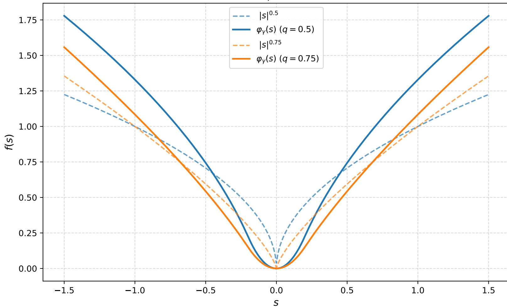
|s|^q vs. \phi_\gamma(s) ( \gamma = 0.2 )
