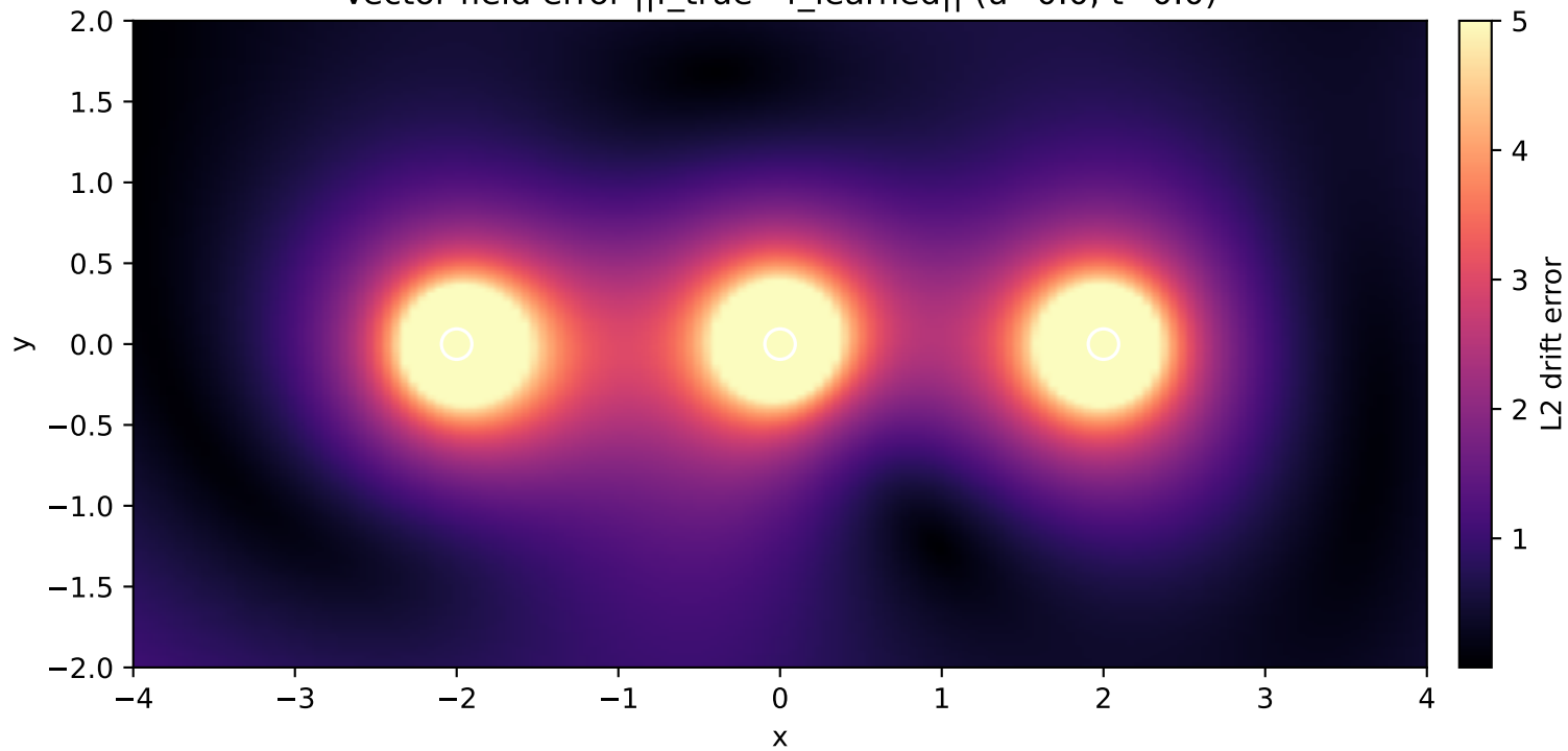
Vector field error ||f\_true - f\_learned|| ( u=0.0 , t=0.0 )
