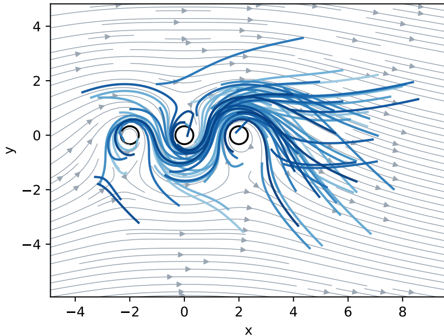
Generated controlled trajectories over stream field
