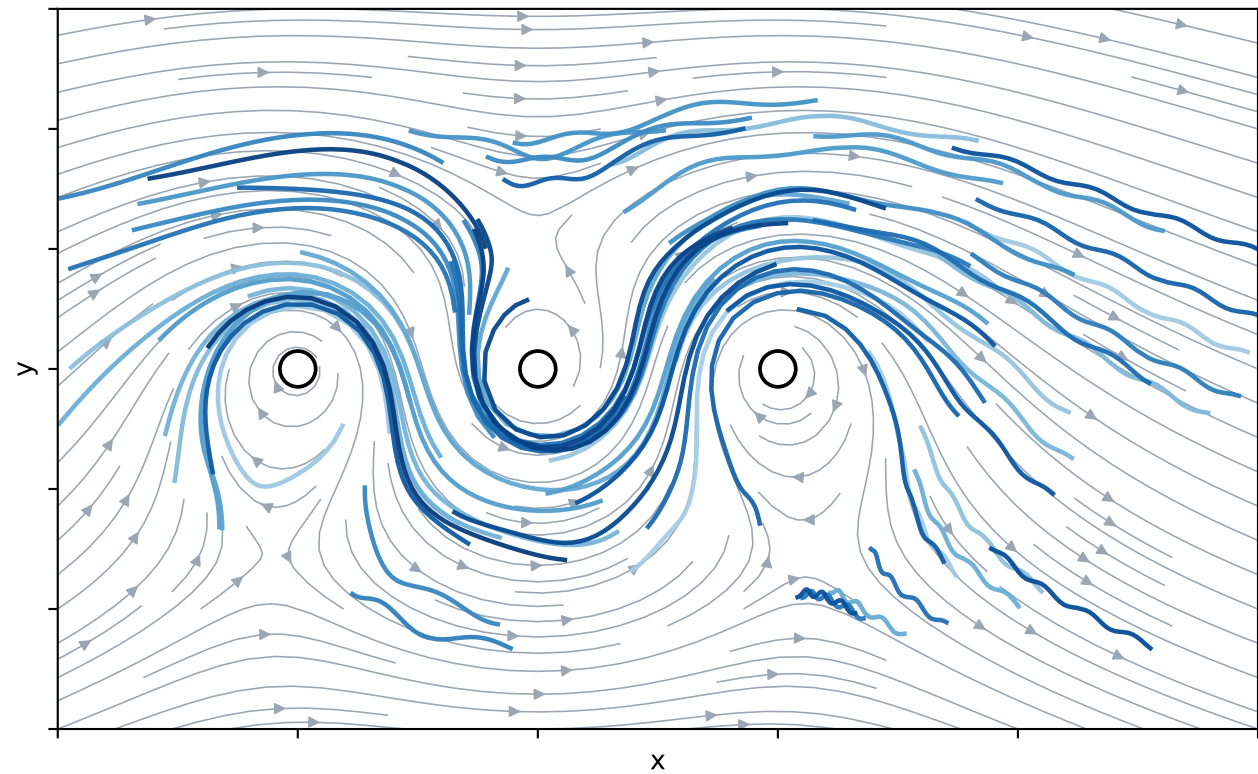
Dataset 2 (sinusoidal)
