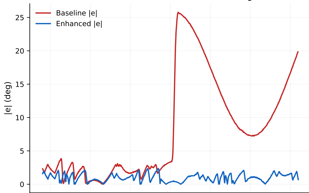
Error near the first critical Nussbaum region
