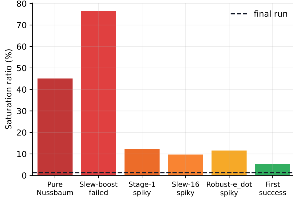
Saturation exposure in failed or over-driven tests
