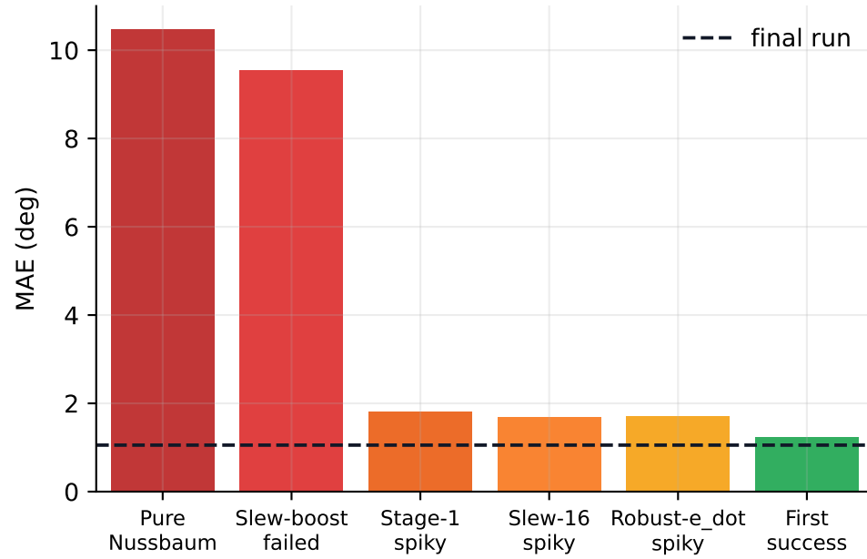
Mean tracking error during rejected/intermediate tests
