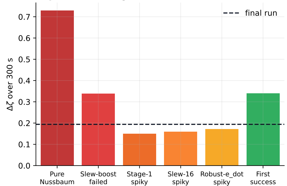
Adaptation-state growth before final containment
