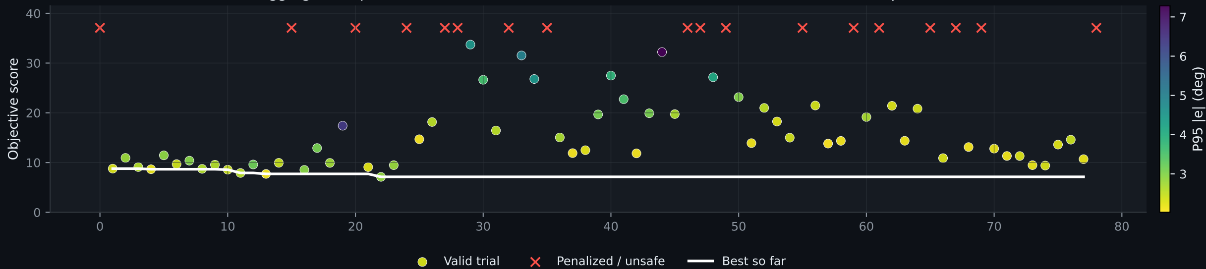
Aggregated Optuna archive: 79 real-hardware trials, 61 valid runs, 87.9 min closed-loop time
