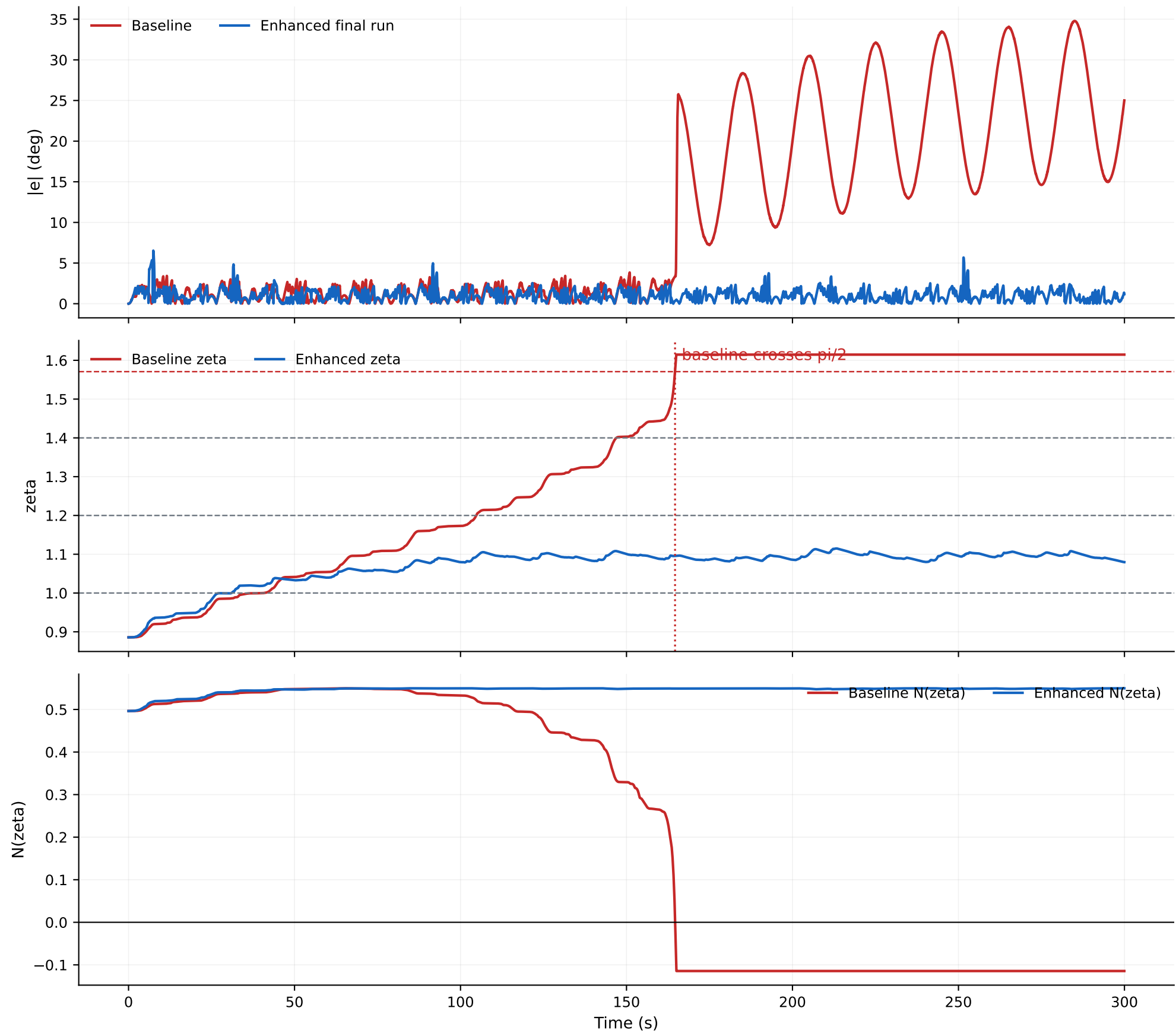
Baseline zeta law versus enhanced Nussbaum controller
