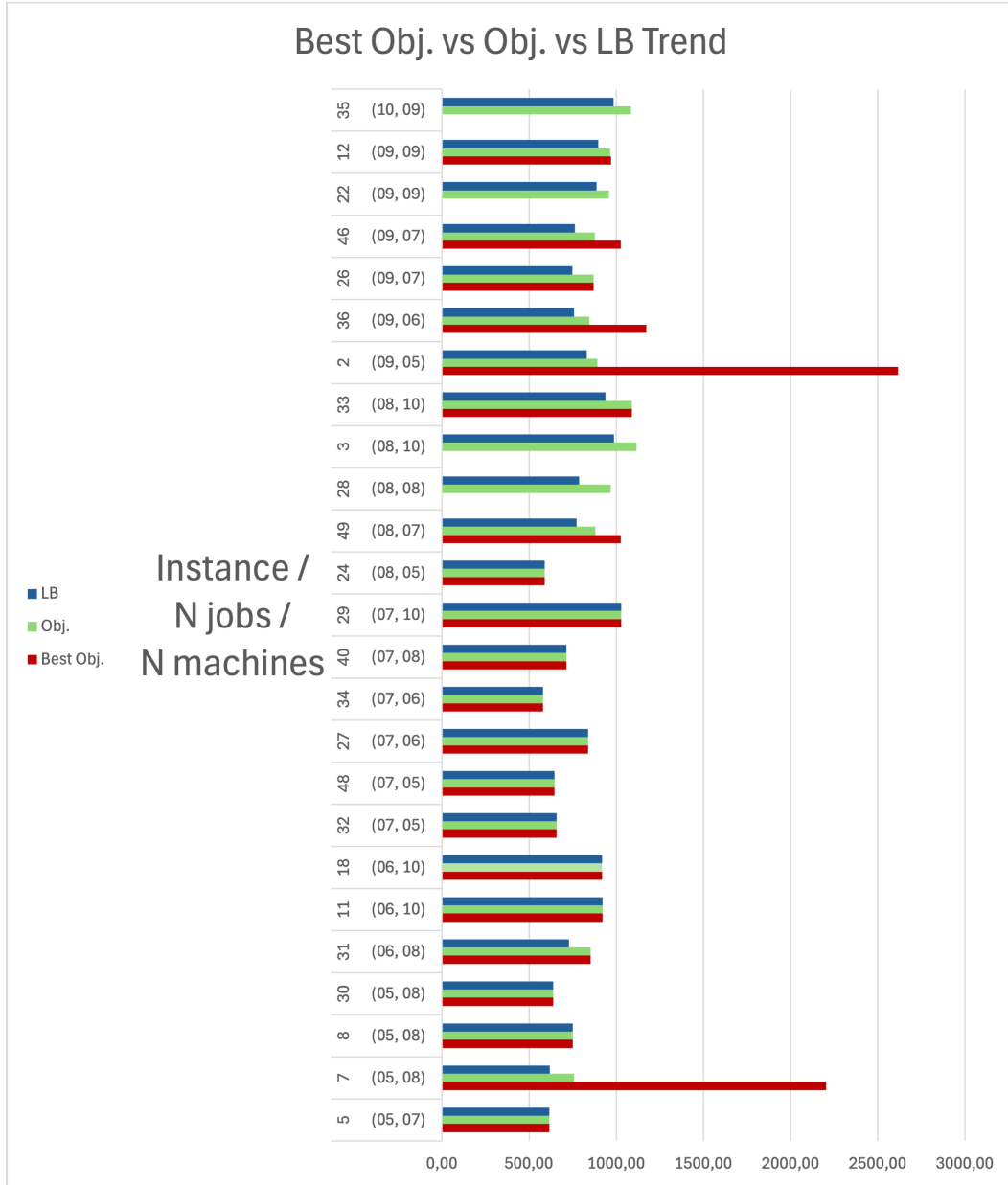
Figure 5.2: Representation of the objective values in an histogram
