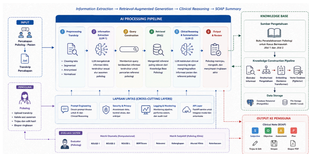
Gambar 3.1 Arsitektur Sistem Clinical Conversation Summarization
