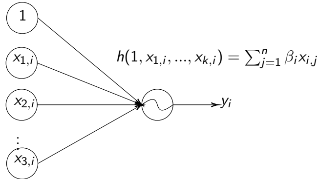
Figura 42.7: \hat{Y}_i = E(Y|X_i = (1, x_{1i}, \dots, x_{pi})^T) = \sum_{j=0}^p \alpha_j x_{ji} con x_{0i} = 1 .
