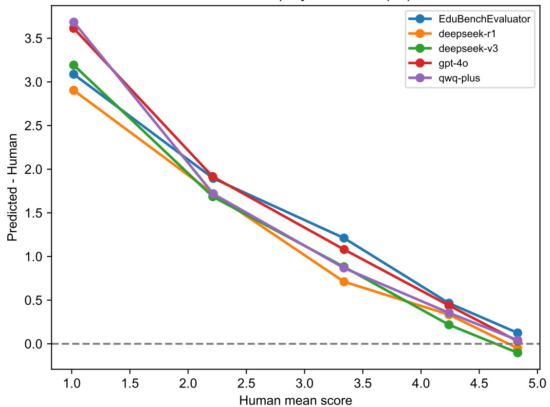
Calibration Gap by Score Bin (en)
