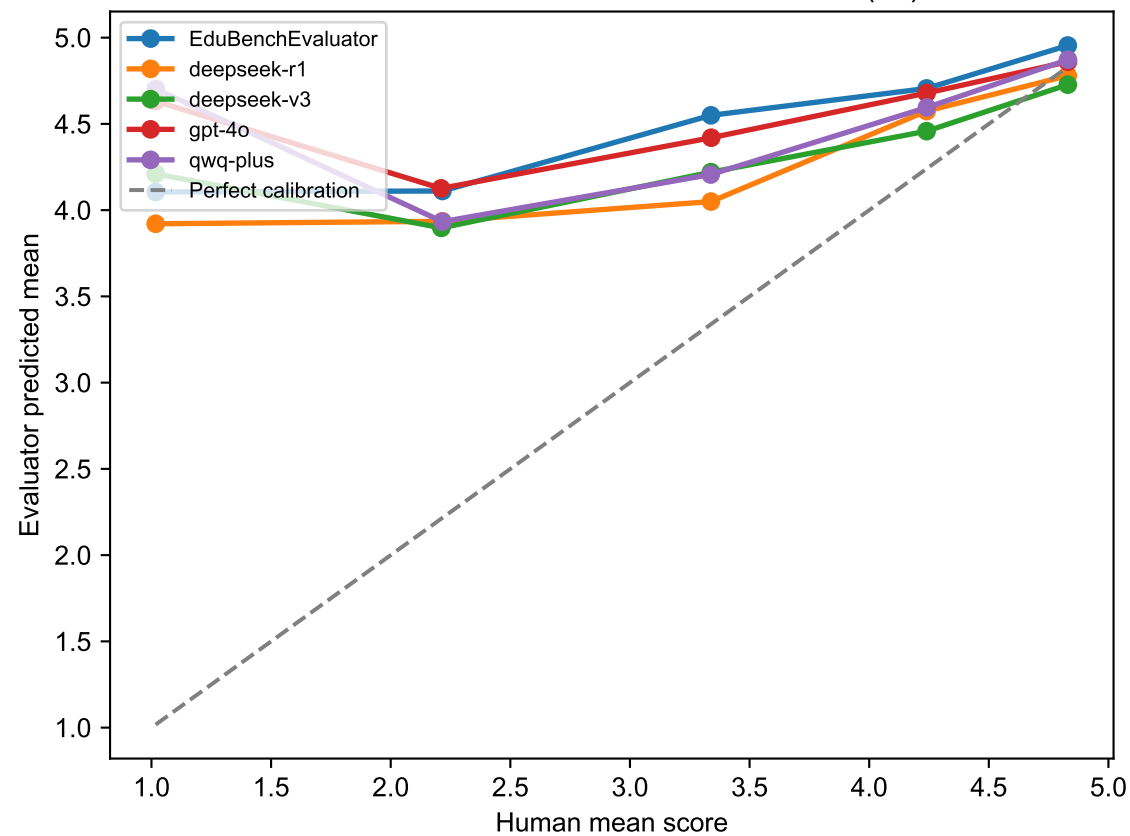
Calibration Curve: Predicted vs Human (en)
