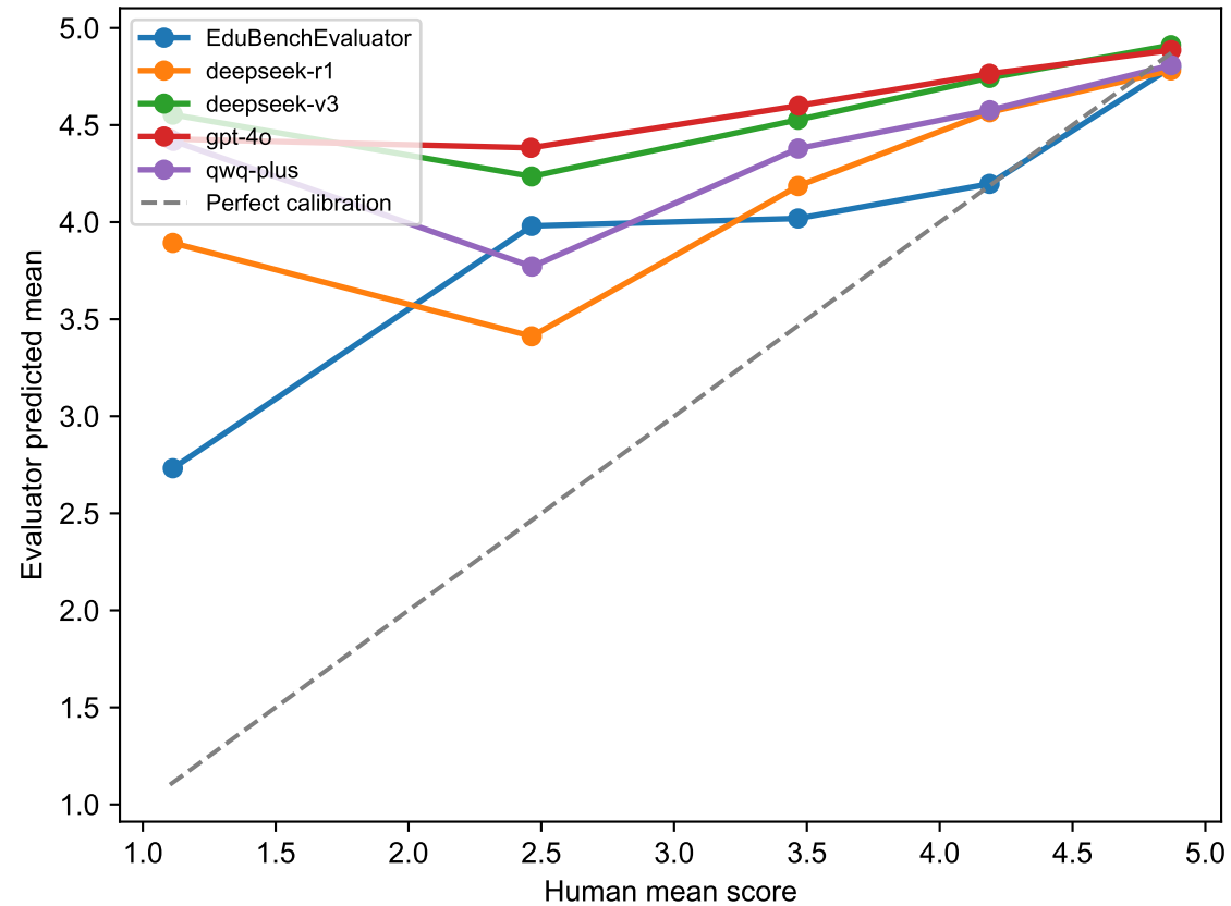
Calibration Curve: Predicted vs Human (zh)
