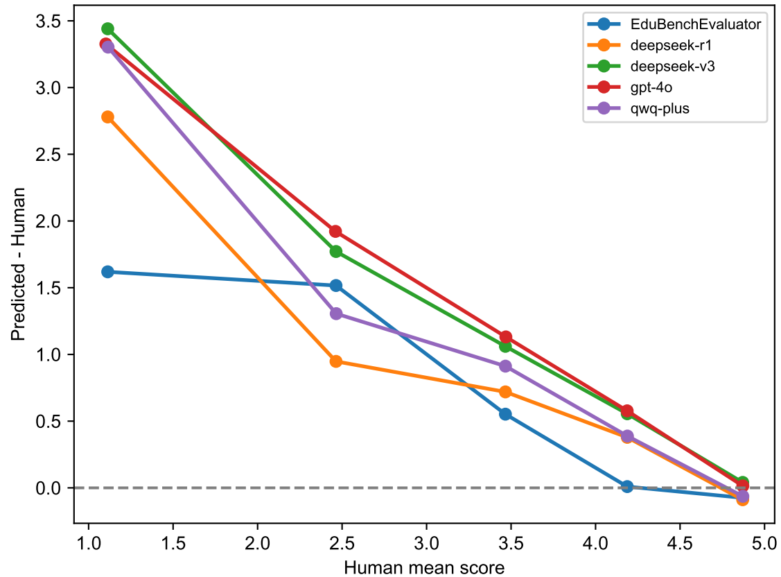
Calibration Gap by Score Bin (zh)
