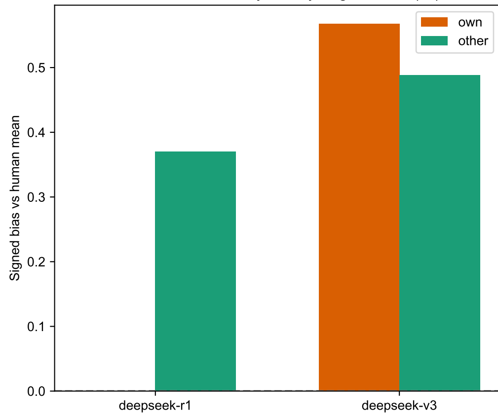
Evaluator Self-Family Affinity: Signed Bias (zh)
