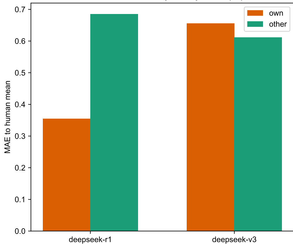
Evaluator Self-Family Affinity: MAE (zh)
