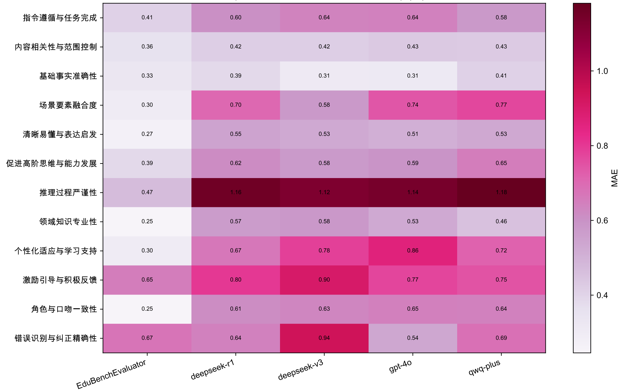
Top-12 Metric × Evaluator MAE Heatmap (zh)
