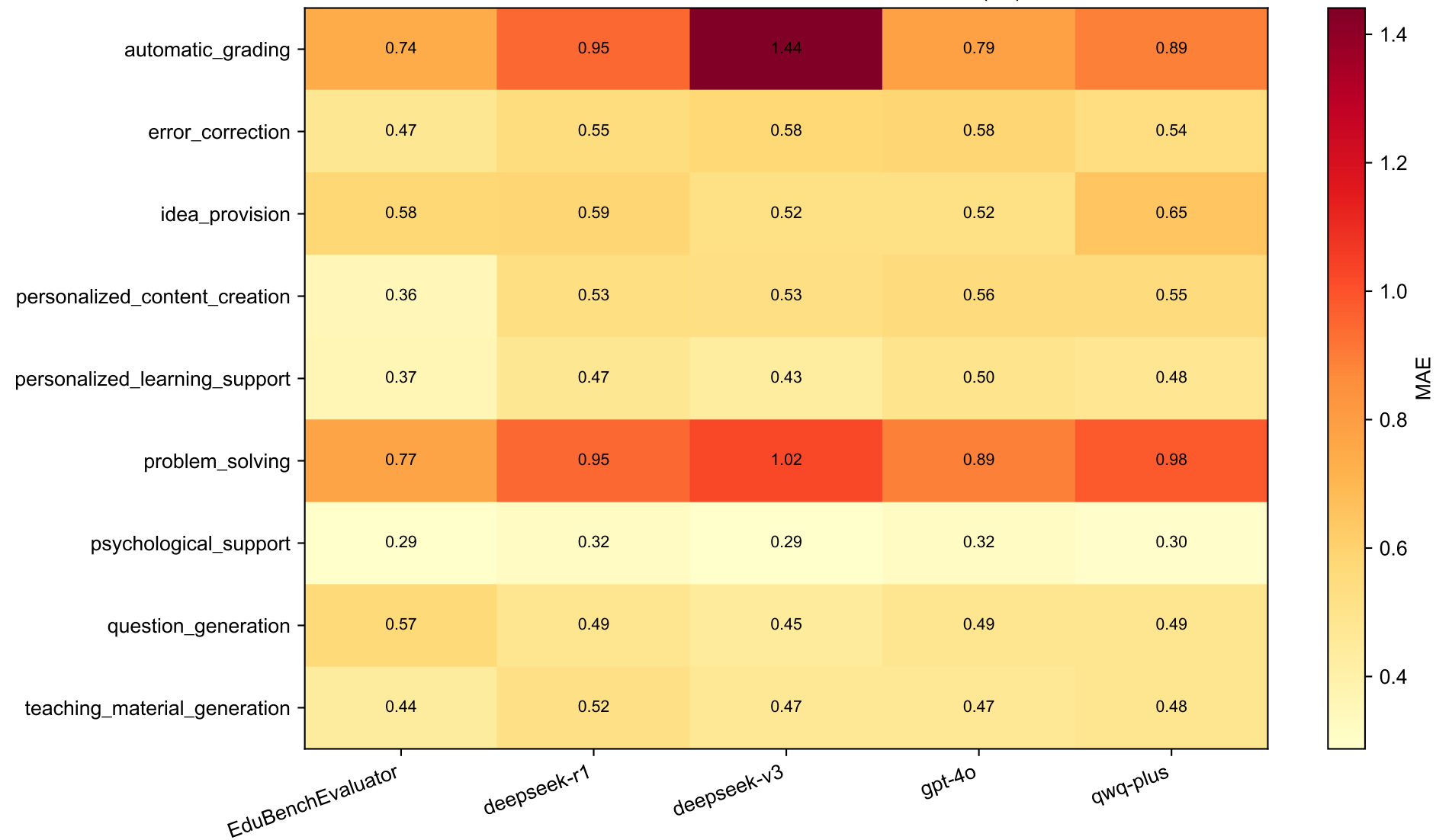
Task × Evaluator MAE to Human Mean (en)
