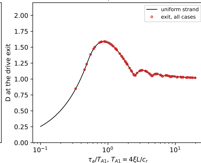
(e) loop, drive exit
