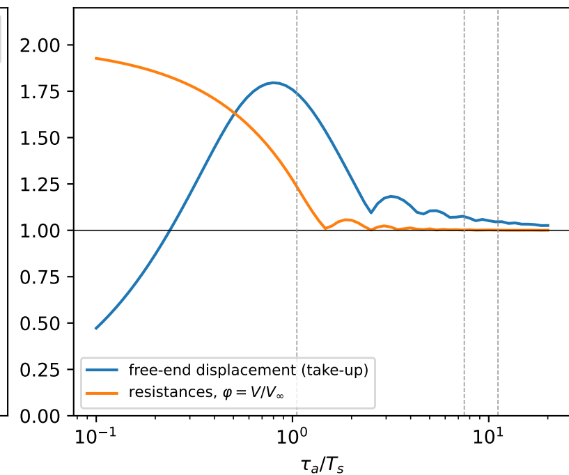
(f) travel and resistances (sine)
