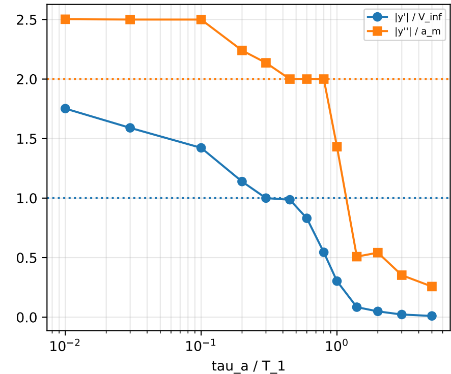
(c) Take-up kinematics, envelope (belt side)
