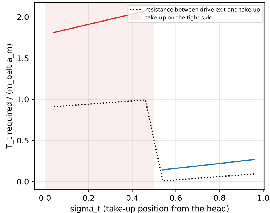
(e) Drive at \sigma = 0.5 (full loop, E = 16 )
