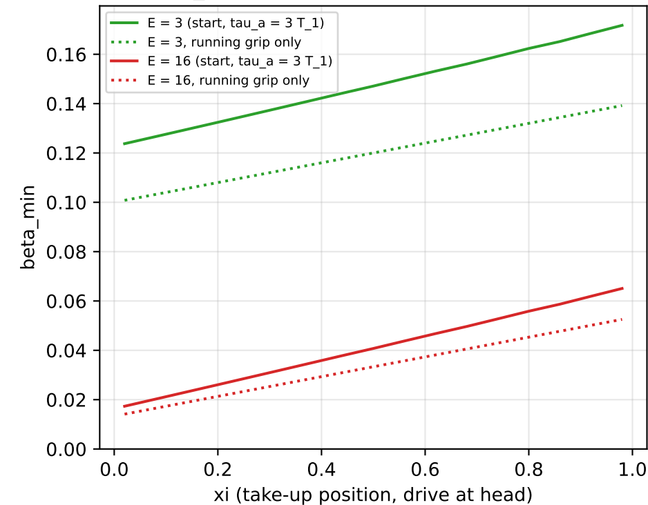
(f) \beta_{\text{min}} , direct counterweight, \gamma = 2
