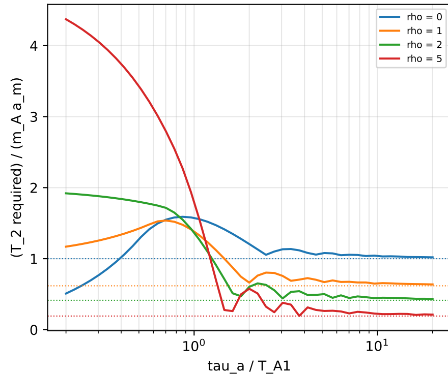
(a) Exit slack, strand A (dotted: slow-start limit)
