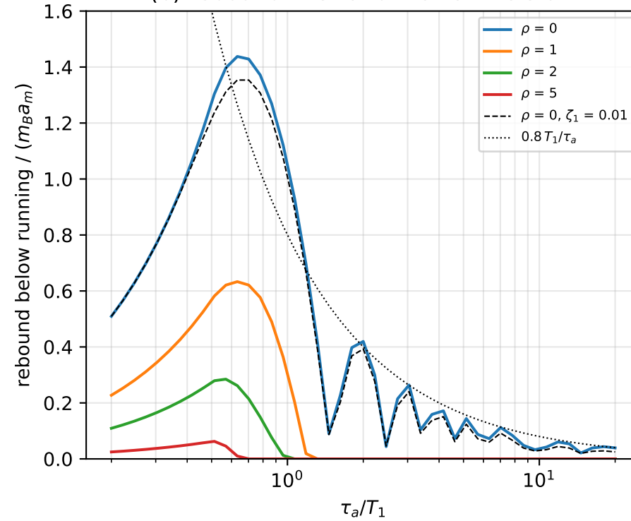
(e) drive at \sigma_d = 0.5 (full loop, E = 16 )
