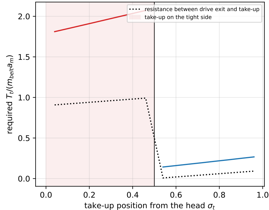
(e) drive at \sigma_d = 0.5 (full loop, E = 16 )
