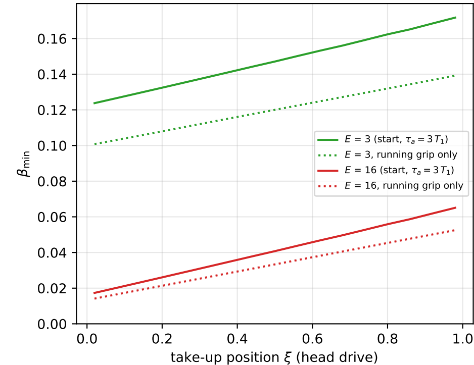
(f) \beta_{min} , direct counterweight, \gamma = 2
