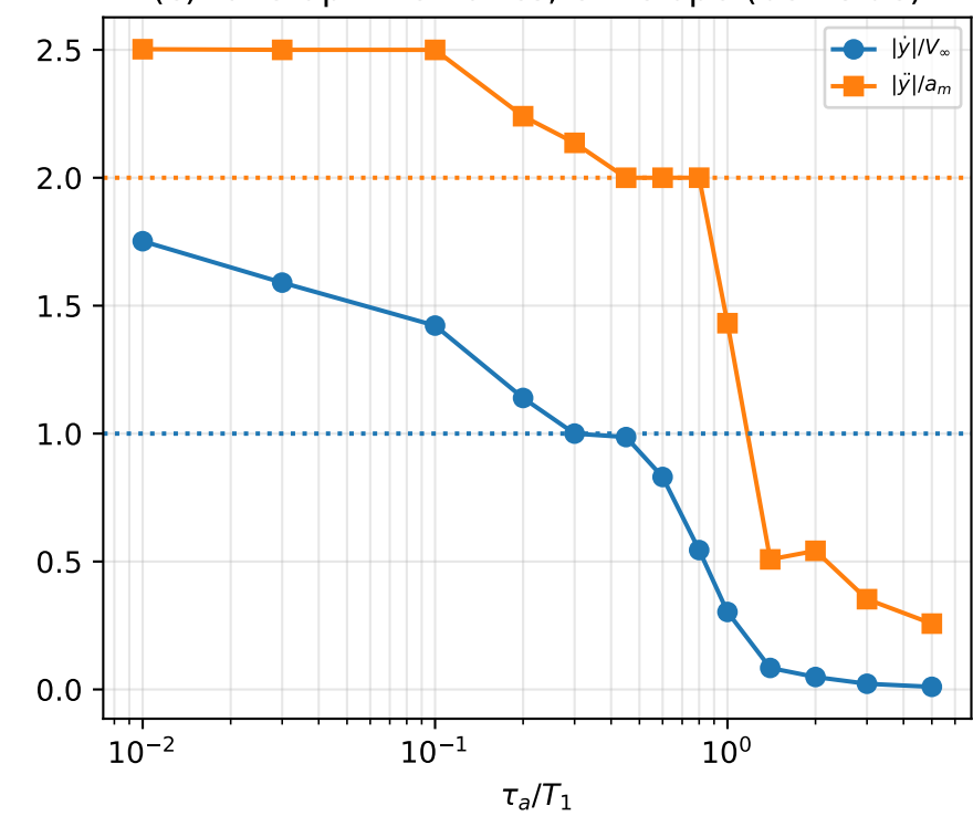
(f) \beta_{min} , direct counterweight, \gamma = 2
