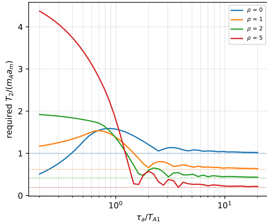
(a) slack at the drive exit, strand A (dotted: slow start)
