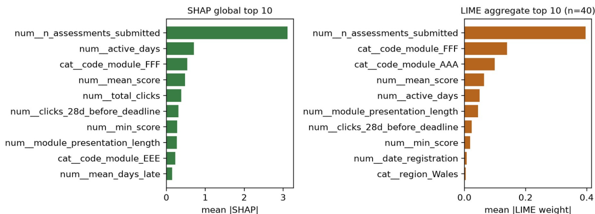
Figure 5.5. SHAP global top 10 (left) and LIME aggregate top 10 (right), shown side by side.
