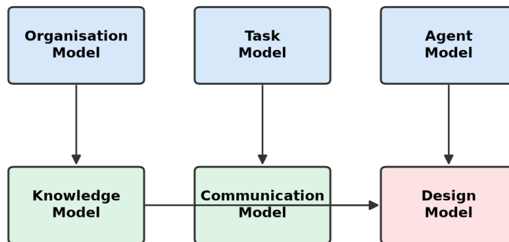
Context models (top) inform knowledge & communication models, which are operationalised in the Design Model (dashboard architecture).
