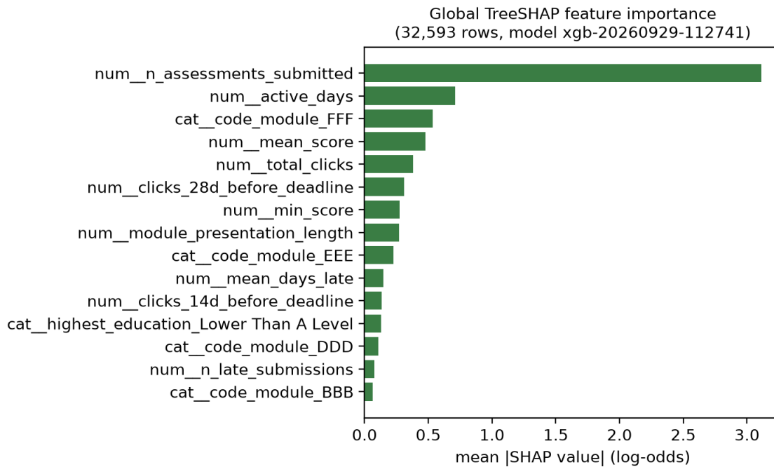
Figure 5.4. Top 15 global TreeSHAP features by mean absolute SHAP value.
