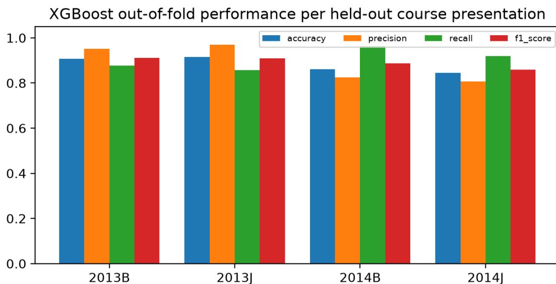
Figure 5.3. XGBoost out-of-fold accuracy, precision, recall, and F1-score for each held-out course presentation.
