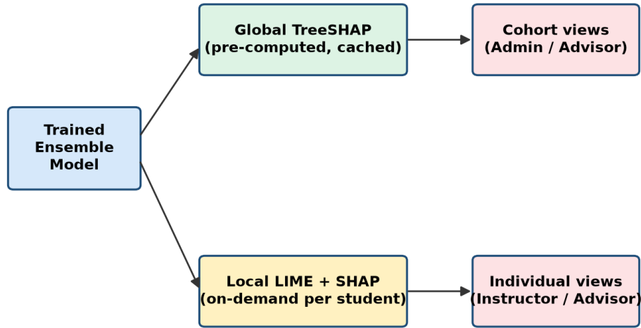
Figure 3.4 Dual-service explainability pipeline (SHAP for global, LIME for local)
