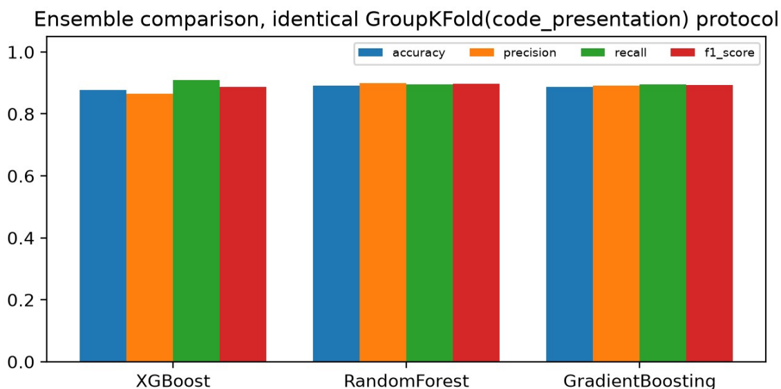
Figure 5.2. XGBoost, Random Forest, and Gradient Boosting compared on the four required metrics under the identical protocol.
