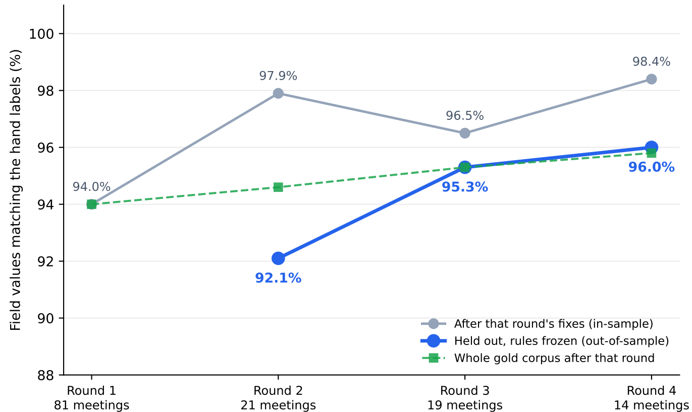
Accuracy across hand-labelling rounds
