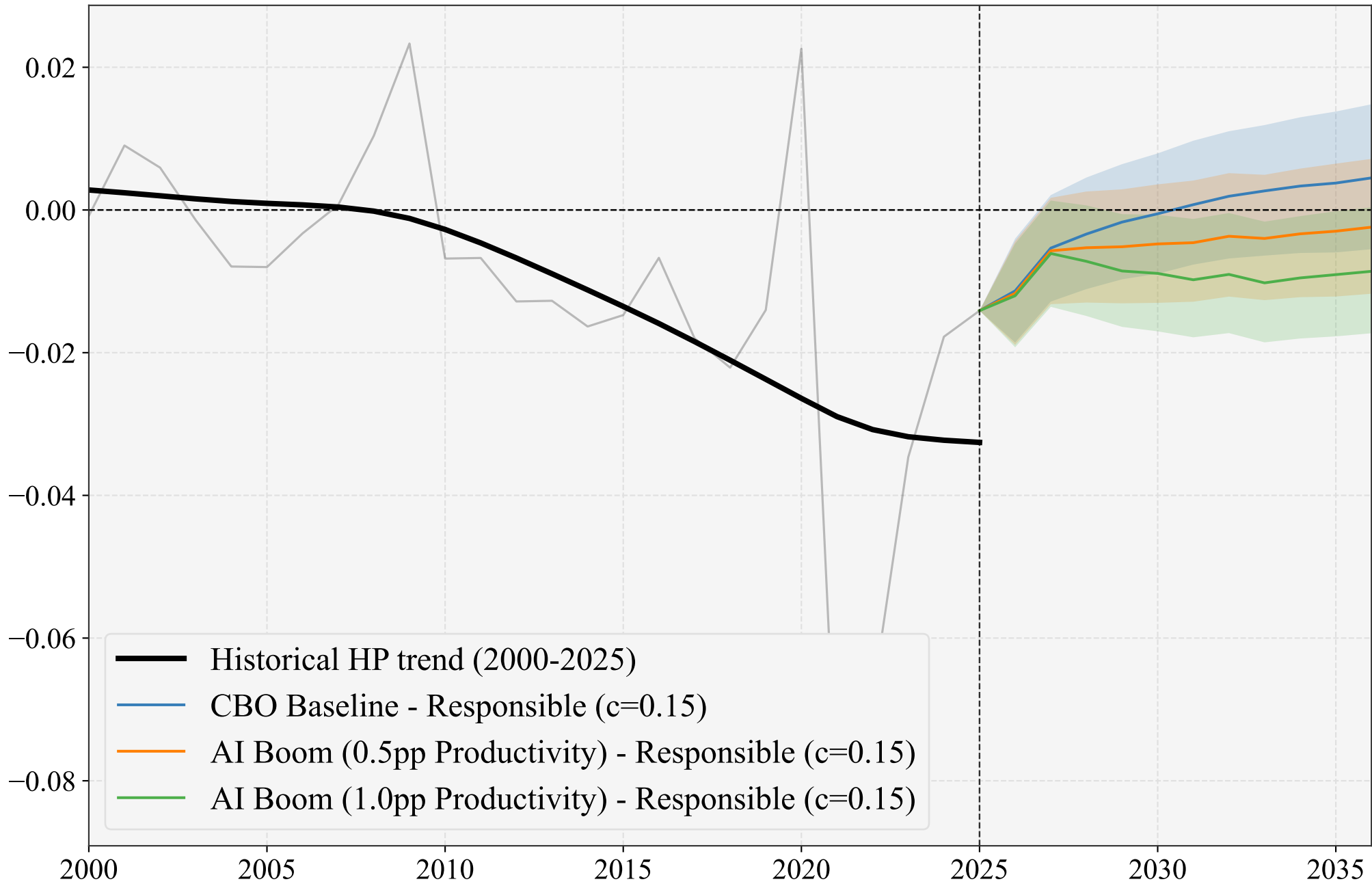
Snowball Term
