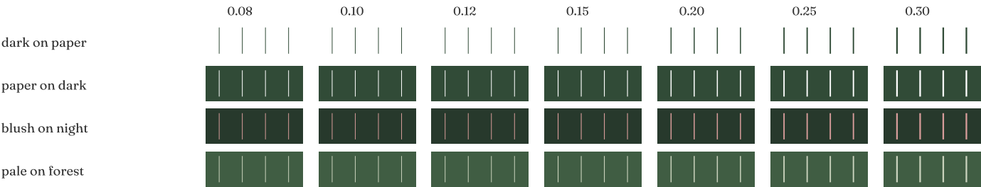
The artwork uses ≥ 0.15 mm for dark lines and ≥ 0.20 mm for light-on-dark lines.
