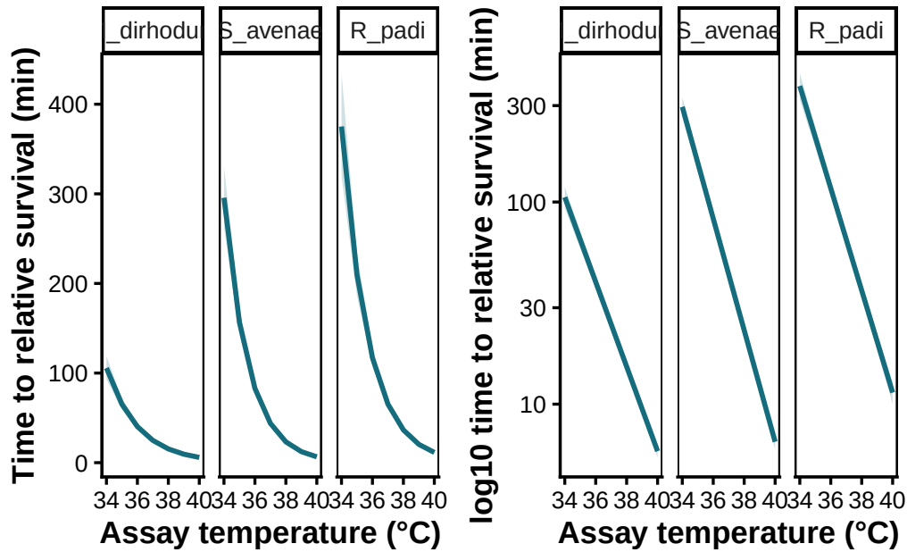
Figure S14: Thermal-death-time curves for the three cereal aphids, read from the joint 4PL posterior across assay temperatures (34–40 °C). Each panel gives the exposure duration needed to reach the relative survival threshold, on a \log_{10} time axis (posterior median with 95% credible band). The slope of each line is -1/z , so a shallower curve means lower thermal sensitivity.
