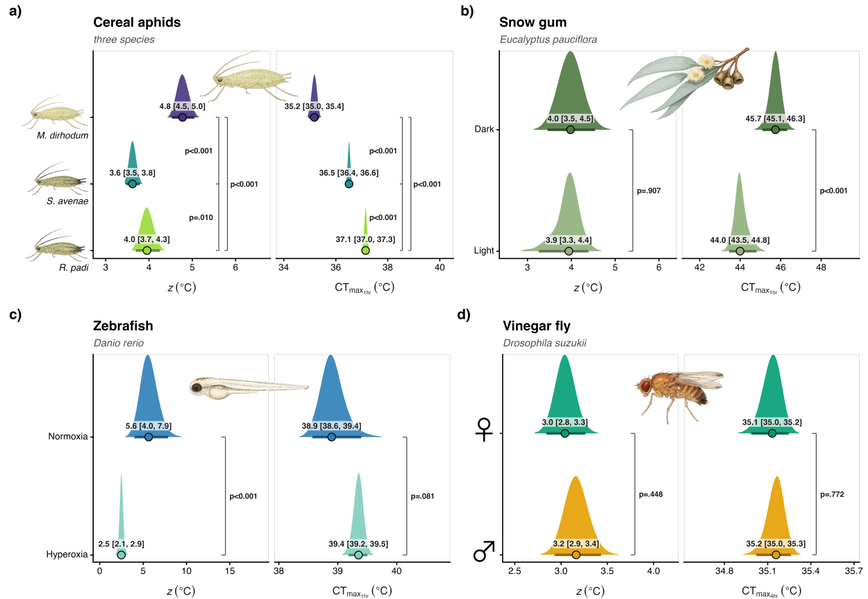
Figure S24: Manuscript Figure 5. Posterior distributions of thermal sensitivity z (left of each panel) and the critical thermal limit CT_{max} (right) from the joint Bayesian 4PL fits for four case studies: a) three cereal-aphid species ( Metopolophium dirhodum , Sitobion avenae , Rhopalosiphum padi ), b) snow gum ( Eucalyptus pauciflora ) leaf photosystem II function under dark vs 90-min-light post-heat recovery, c) zebrafish ( Danio rerio ) larvae under normoxia vs hyperoxia, and d) the vinegar fly ( Drosophila suzukii ) by sex. Filled ridges are the posterior densities, coloured by group; the black-outlined point and bar give the posterior median and 95% credible interval, also printed beside each ridge. The CT_{max} reference exposure follows each study's own analysis: 1 h for aphids, snow gum, and zebrafish (relative midpoint threshold) and 4 h for the vinegar fly (absolute LT50, following Ørsted et al. (2024)). Within each panel the groups are fit jointly, so pairwise posterior contrasts are annotated as brackets labelled with the pMCMC (twice the smaller posterior tail probability of the difference; smaller values indicate stronger evidence the groups differ). Panels carry independent x-axes.
