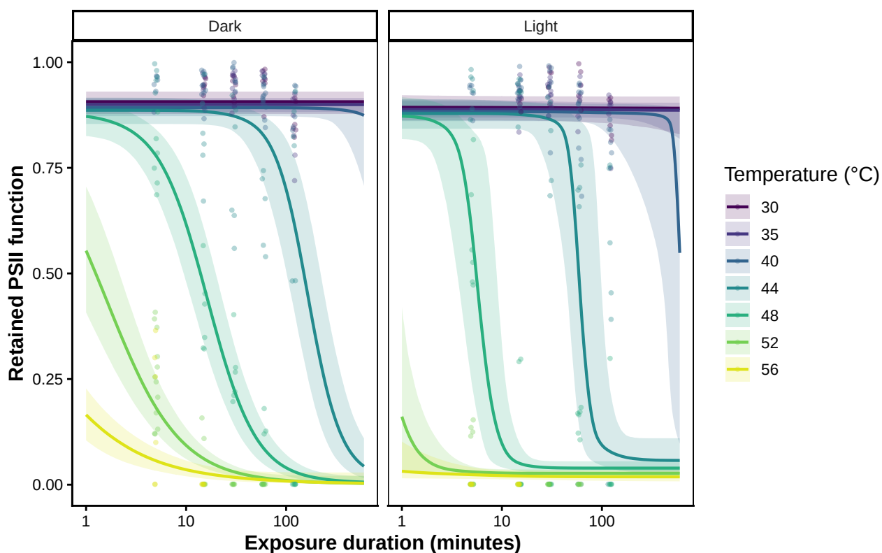
Figure S16: Fitted retained-PSII-function surfaces for snow gum under dark and light post-heat recovery (posterior median and 95% credible band), with observed per-replicate proportions overlaid. The light-recovery curves cross the midpoint at shorter durations, the visual signature of the lower CT_{max} .
