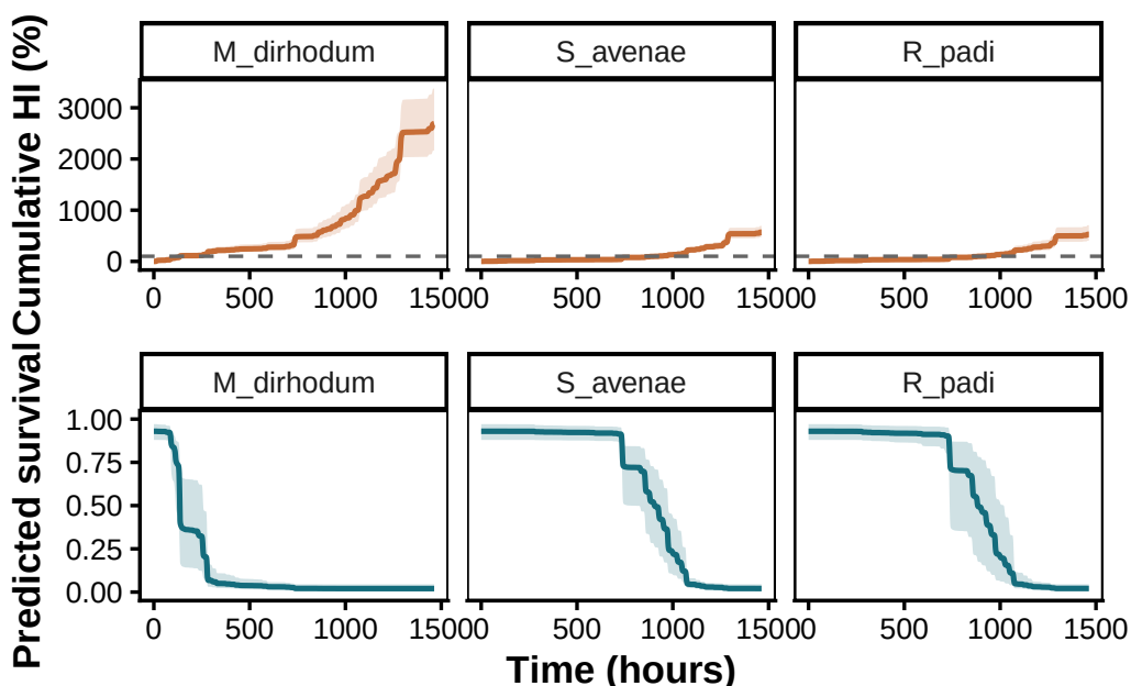
Figure S15: Multi-group heat-injury projection. Cumulative heat injury (100% = one LT_{50} dose) and predicted survival for the three aphid species under the unmodified Wuhan May–June 2016 hourly temperature trace, from a single predict_heat_injury(by = "species") call.
