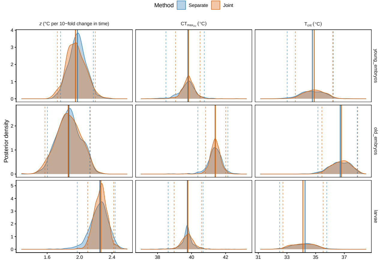
Figure S36: Posterior densities of z (left), CT_{max1hr} (middle), and T_{crit} (right) for each zebrafish life stage, separate-fit (blue) vs joint-fit (orange). Solid vertical lines mark the posterior median; dashed lines mark the 95 % credible interval.
