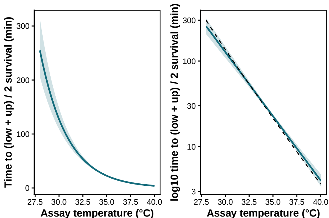
Figure S6: Posterior LT50(T) curve (median + 95% CrI, blue) recovered by derive_tdt_curve() from the T -varying fit, with the analytical truth overlaid (dashed black). The curve is visibly bent rather than straight in T , and the posterior tracks the truth.
