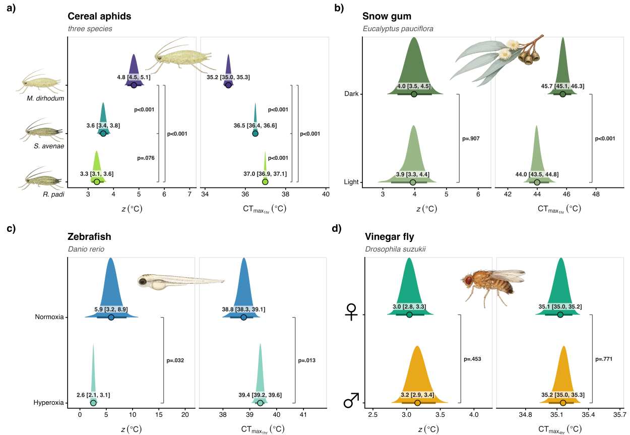
Figure S22: Manuscript Figure 5. Posterior distributions of thermal sensitivity z (left of each panel) and the critical thermal limit CT_{\max} (right) from the joint Bayesian 4PL fits for four case studies: a) three cereal-aphid species ( Metopolophium dirhodum , Sitobion avenae , Rhopalosiphum padi ), b) snow gum ( Eucalyptus pauciflora ) leaf photosystem II function under dark vs 90-min-light post-heat recovery, c) zebrafish ( Danio rerio ) larvae under normoxia vs hyperoxia, and d) the vinegar fly ( Drosophila suzukii ) by sex. Filled ridges are the posterior densities, coloured by group; the black-outlined point and bar give the posterior median and 95% credible interval, also printed beside each ridge. The CT_{\max} reference exposure follows each study's own analysis: 1 h for aphids, leaf and zebrafish (relative midpoint threshold) and 4 h for the vinegar fly (absolute LT50, following Ørsted et al. (2024)). Within each panel the groups are fit jointly, so pairwise posterior contrasts are annotated as brackets labelled with the pMCMC (twice the smaller posterior tail probability of the difference; smaller values indicate stronger evidence the groups differ). Panels carry independent x-axes.
