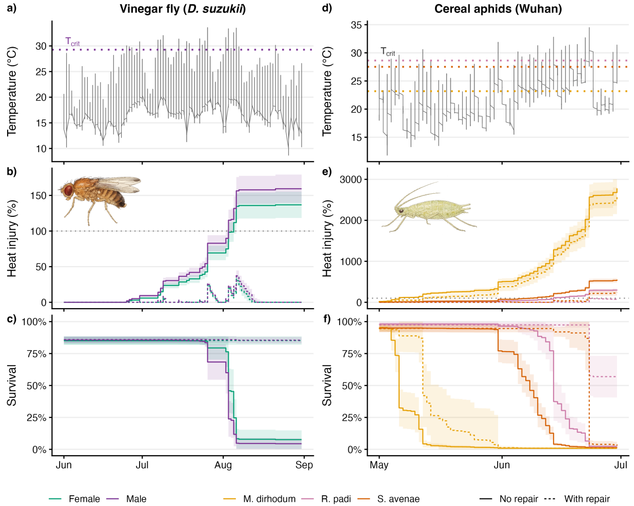
Figure S23: Manuscript Figure 6. Heat-injury accumulation and predicted survival under field temperature trajectories for the vinegar fly ( Drosophila suzukii , by sex; panels a-c) and three cereal aphids ( Metopolophium dirhodum , Sitobion avenae , Rhopalosiphum padi ; panels d-f). (a, d) the temperature trace — shaded NicheMapR (Kearney & Porter 2017) microclimate temperature for the fly (Rennes, France, Jun–Aug 2018; Ørsted et al. (2024)) and the hourly air-temperature trace for the aphids (Wuhan, May–June 2016; Li et al. (2023), Open-Meteo ERA5 reanalysis) — with the critical temperature threshold T_{crit} (dotted line). (b, e) cumulative heat injury (100% = one LT_{50} dose, dotted grey) and (c, f) predicted survival, each with and without damage repair (line type). Fly panels are coloured by sex, aphid panels by species. Bands are \pm 1 SE across posterior draws. Predicted survival begins at each group’s fitted upper asymptote rather than at 100% (the vinegar-fly 4PL estimates a maximum survival of 85%, up < 1 ). Repair uses an illustrative Sharpe–Schoolfield kernel with an Arrhenius (uninhibited) rate scale r_{ref} = 0.005 LT_{50} -dose h^{-1} ; it is not empirically fitted.
