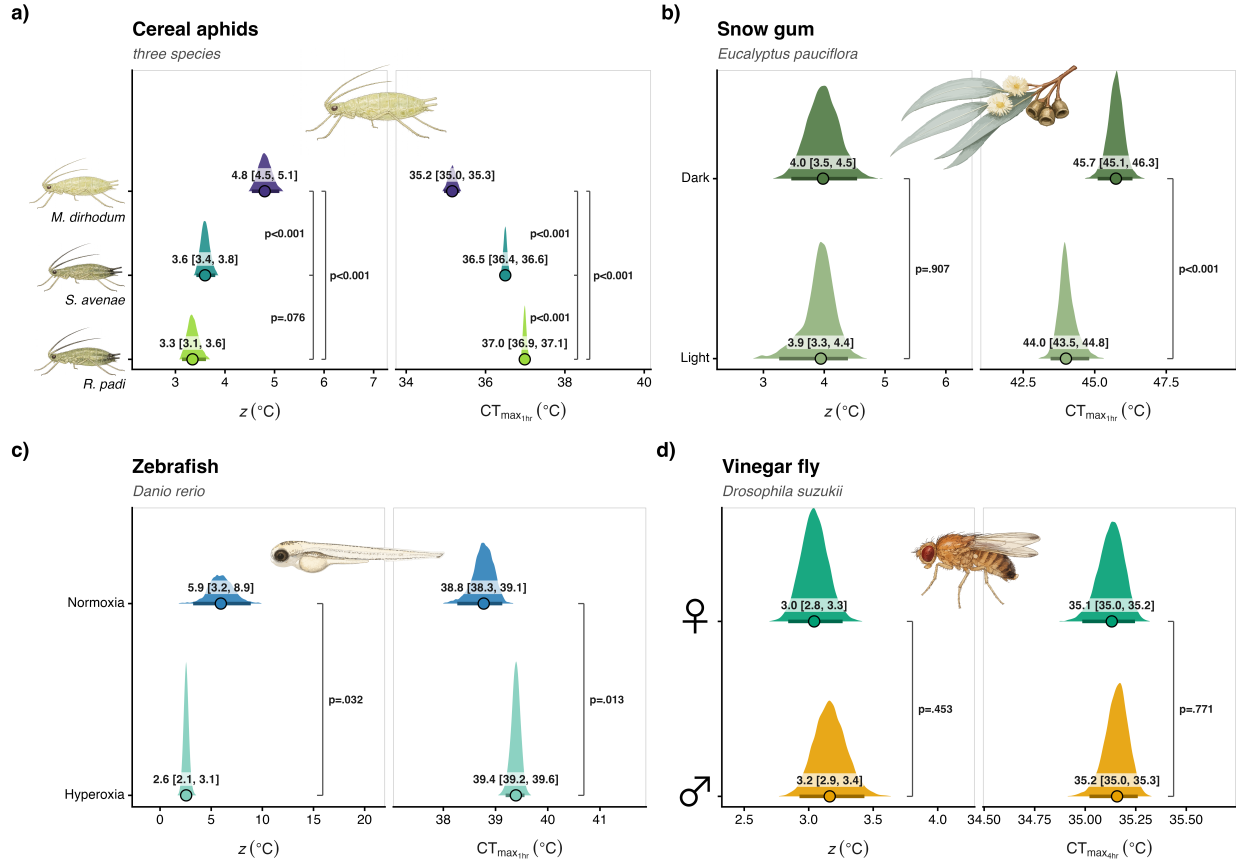
Figure S22: Manuscript Figure 5. Posterior distributions of thermal sensitivity z (left of each panel) and the critical thermal limit CT_{max} (right) from the joint Bayesian 4PL fits for four case studies: a) three cereal-aphid species ( Metopolophium dirhodum , Sitobion avenae , Rhopalosiphum padi ), b) snow gum ( Eucalyptus pauciflora ) leaf photosystem II function under dark vs 90-min-light post-heat recovery, c) zebrafish ( Danio rerio ) larvae under normoxia vs hyperoxia, and d) the vinegar fly ( Drosophila suzukii ) by sex. Filled ridges are the posterior densities, coloured by group; the black-outlined point and bar give the posterior median and 95% credible interval, also printed beside each ridge. The CT_{max} reference exposure follows each study's own analysis: 1 h for aphids, leaf and zebrafish (relative midpoint threshold) and 4 h for the vinegar fly (absolute LT50, following Ørsted et al. (2024)). Within each panel the groups are fit jointly, so pairwise posterior contrasts are annotated as brackets labelled with the pMCMC (twice the smaller posterior tail probability of the difference; smaller values indicate stronger evidence the groups differ). Panels carry independent x-axes.
