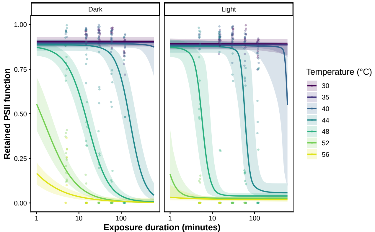
Figure S14: Fitted retained-PSII-function surfaces for snow gum under dark and light post-heat recovery (posterior median and 95% credible band), with observed per-replicate proportions overlaid. The light-recovery curves cross the midpoint at shorter durations, the visual signature of the lower CT_{max} .
