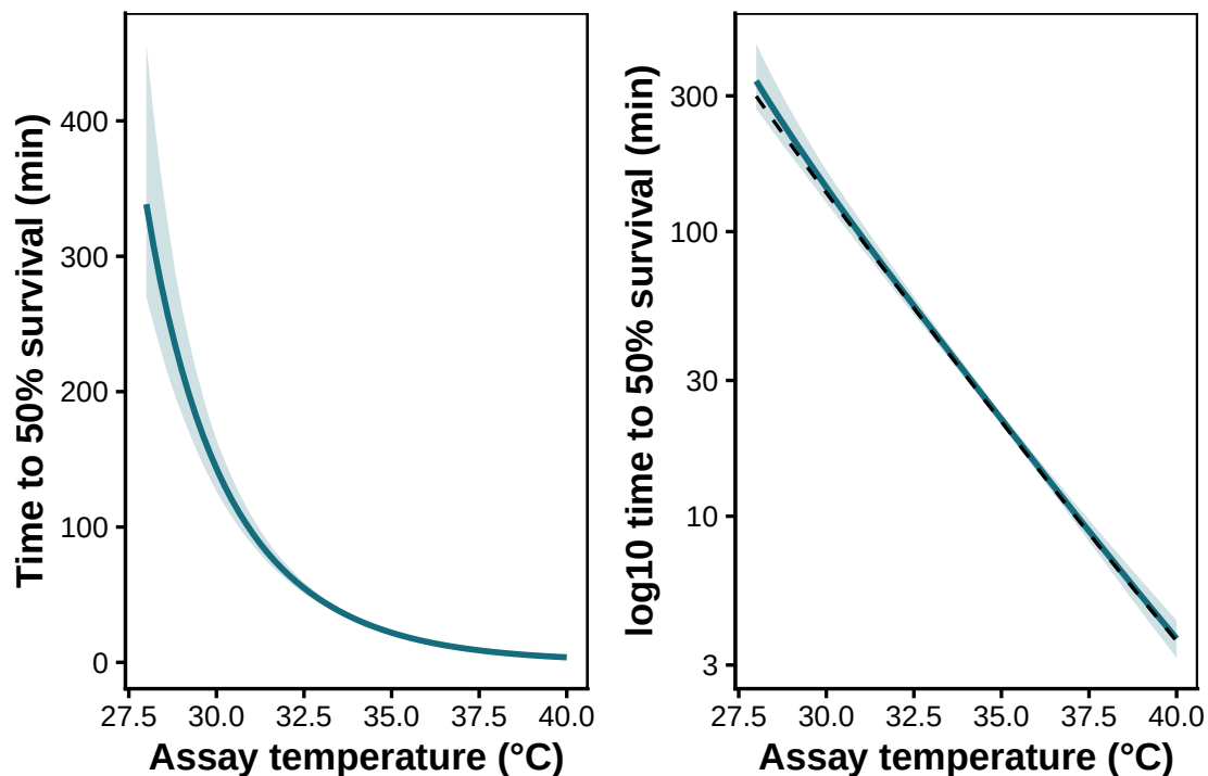
Figure S7: Posterior LT50(T) curve (median + 95% CrI, blue) recovered by derive_tdt_curve() from the T -varying fit, with the analytical truth overlaid (dashed black). The curve is visibly bent rather than straight in T , and the posterior tracks the truth.
