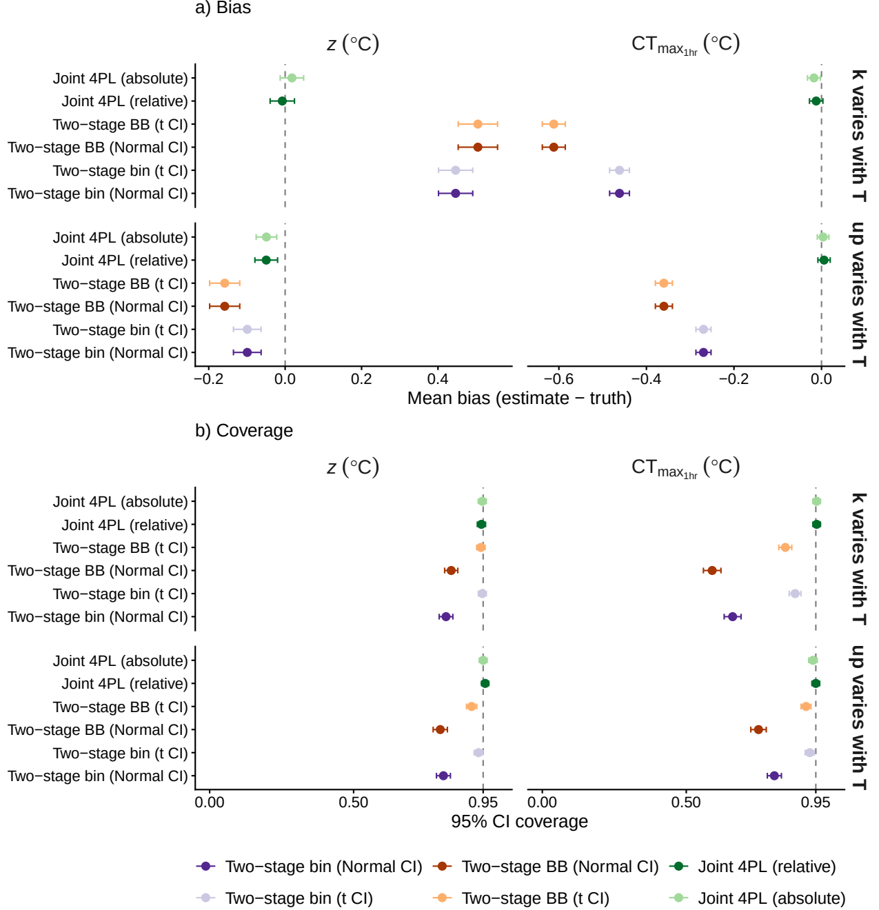
Figure 2: Simulation performance when the data-generating process violates classical TDT shape assumptions. Row labelled ‘ up varies with T ’: upper asymptote up declines 0.01 per ^{\circ}\text{C} from 0.92 at T = 34^{\circ}\text{C} , with low = 0.05 and k = 8 constant in T . Row labelled ‘ k varies with T ’: slope k ranges from 7 at 30^{\circ}\text{C} to 9 at 38^{\circ}\text{C} , with up = 0.92 and low = 0.05 constant. Both rows use 5 replicate vials per ( T \times duration) cell, N_{sim} = 1000 simulated datasets per row, and beta-binomial overdispersion ( \phi = 5 ). Panel a): mean signed bias in z (left column) and CT_{\max_{1hr}} (right column) with 95% Monte Carlo uncertainty intervals (mean \pm 1.96 MCSE). Panel b): 95% interval coverage with the same column layout. Dashed lines mark zero bias and nominal coverage. Two-stage Normal- and t-quantile variants share point estimates and differ only in Stage-2 delta-method interval construction. 4PL = four-parameter log-logistic, BB = beta-binomial, bin = binomial, CI = credible interval.
