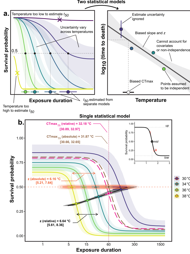
Figure 1: Conceptual comparison of the classical two-stage TDT/TLS workflow and the joint Bayesian four-parameter log-logistic (4PL) model. (a) In the two-stage workflow, separate dose-response curves are fit at each assay temperature and the resulting t_{50} estimates are regressed against temperature. This workflow can fail when assays do not bracket t_{50} , treats first-stage estimates as fixed and independent, and does not naturally propagate uncertainty, covariates, or hierarchical structure into z and CT_{max_{1hr}} . (b) The joint 4PL model estimates the full survival surface in one model. Coloured curves show posterior median survival probabilities at assay temperatures, with shaded pointwise 95% credible intervals. Filled circles mark the model midpoint, mid(T) , defining relative \log_{10} t_{50} ; open triangles mark the absolute 50% survival crossing. A relative threshold is each curve's own midpoint (halfway between its lower and upper asymptotes), whereas an absolute threshold is a fixed survival probability (here 50%); the two coincide only when the asymptotes are 0 and 1 (see Methods). The black and steelblue trajectories give the relative and absolute t_{50} relationships used to derive z_{rel} , z_{abs} , and CT_{max_{1hr}} at the 60-min reference. Dashed curves show the fitted dose response at the corresponding relative and absolute CT_{max_{1hr}} values. Inset: the 4PL parameters low , up , mid , and k . Values are illustrative.
