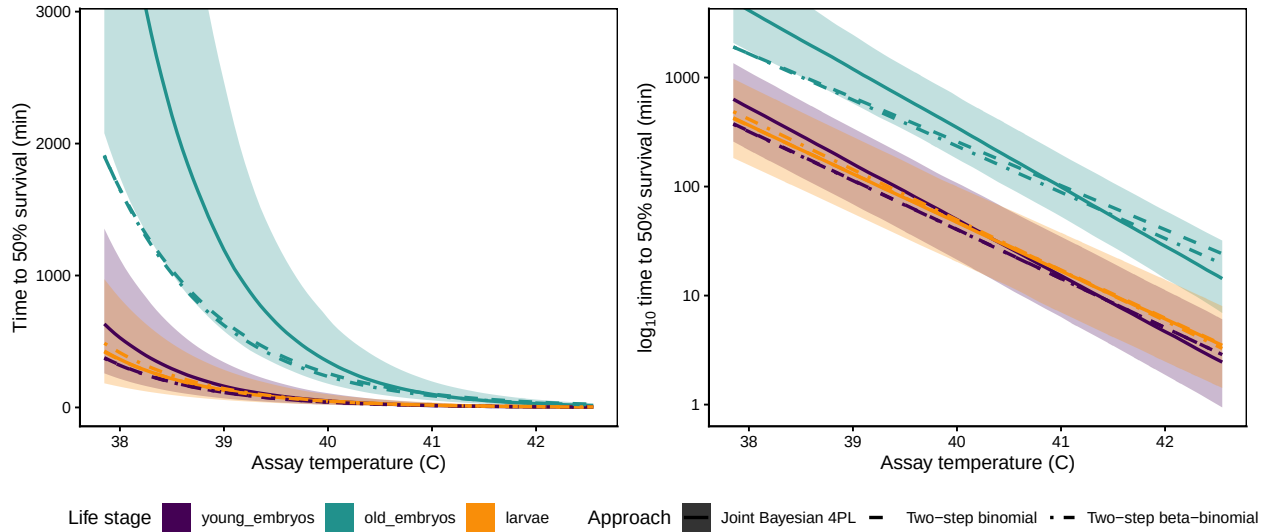
Figure S37: Zebrafish TDT-line comparison between the joint 4PL and the classical two-stage fits. The joint 4PL posterior median and 95 % credible band are repeated from Figure S35; two-stage lines are point-estimate regressions from binomial and beta-binomial Stage-1 fits.
