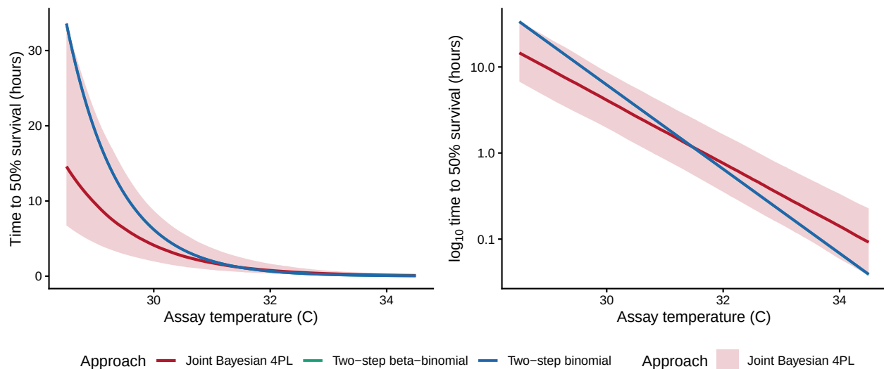
Figure S22: Brown shrimp TDT-line comparison. The joint 4PL posterior median and 95 % credible band are repeated from Figure S20; the two classical two-stage lines are overlaid as point-estimate regressions.
