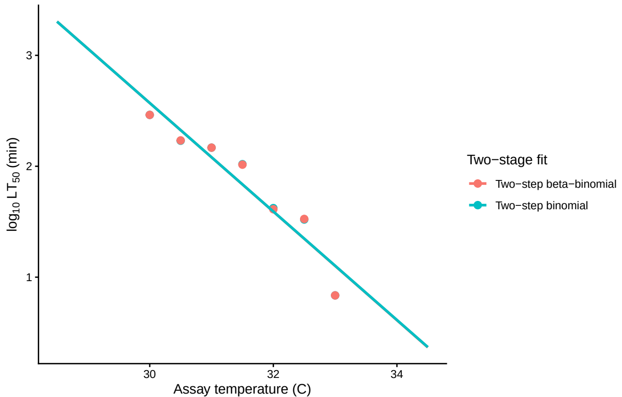
Figure S16: Classical two-stage TDT lines for brown shrimp. Points are Stage-1 \log_{10} LT 50 estimates; lines are the Stage-2 regressions. The beta-binomial Stage-1 fit allows overdispersion within each assay temperature, but both approaches reduce to a single point estimate per temperature for Stage 2.
