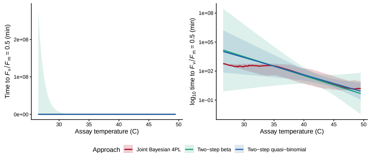
Figure S45: Snow gum leaf PSII TDT-line comparison at a common absolute threshold ( F_v/F_m = 0.5 ). The joint 4PL posterior median and 95% credible band are the time to F_v/F_m = 0.5 ( target_surv = "absolute" ) — the only threshold the forced-0/1 two-stage can target; the two classical two-stage lines are overlaid with their pointwise 95% confidence bands from predict.lm() on the Stage-2 regression (Stage-1 LT50s treated as known points). Outside the assayed 28–48 °C window both methods extrapolate.
