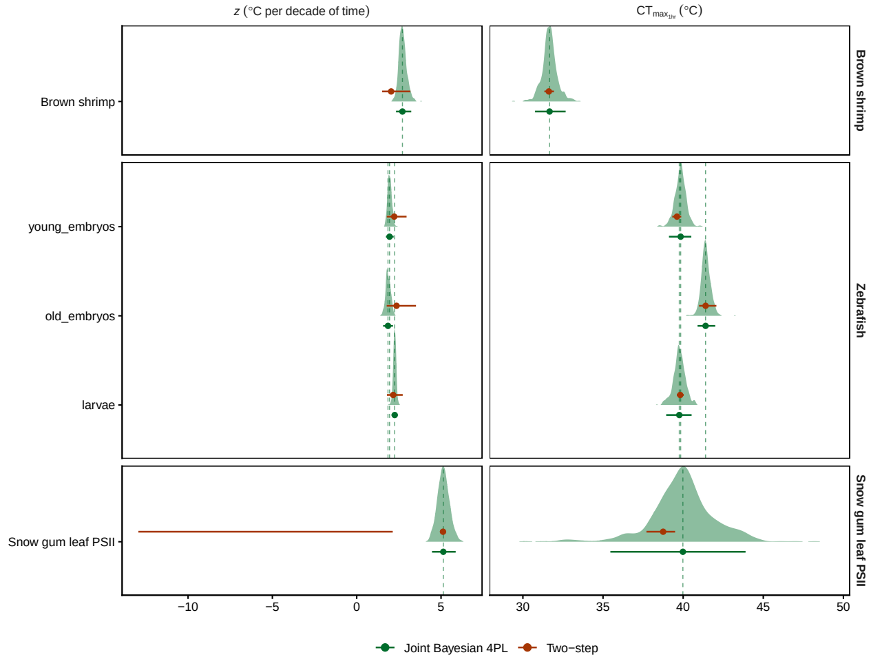
Figure S52: Manuscript Figure 4. Posterior densities of z (left column) and CT_{max1hr} (right column) from the joint Bayesian 4PL fits (green ridges, #006d2c) for the three case studies (rows). The 4PL posterior median and 95% credible interval are overlaid as a green pointrange. The classical two-stage point estimate (beta-binomial Stage 1 for the brown shrimp and zebrafish counts, beta Stage 1 for the snow gum leaf PSII proportions) is shown for comparison as an orange pointrange (median + 95% CI, #a63603). Dashed vertical lines mark the 4PL posterior median for each entity. The zebrafish panel splits into three ridges, one per life stage.
