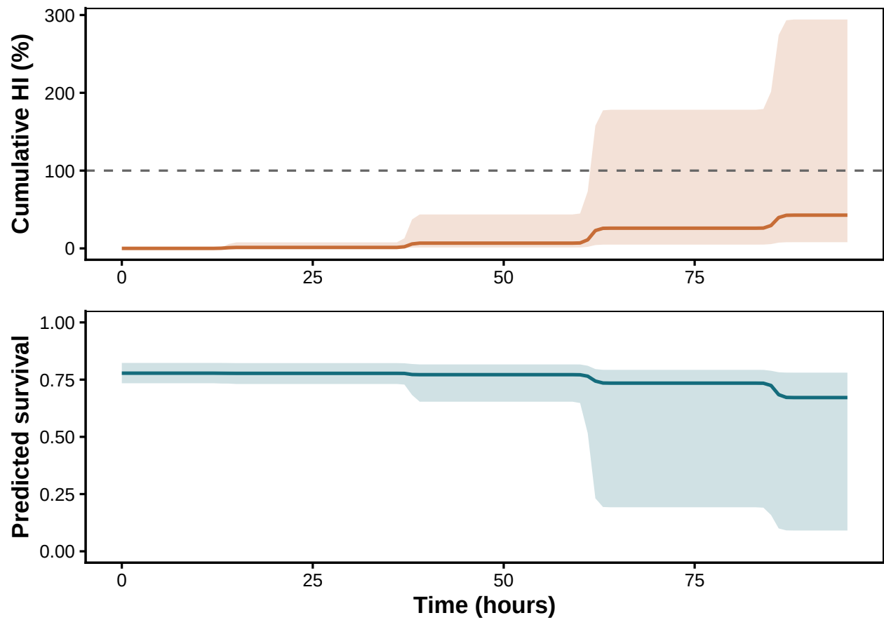
Figure S50: 4-day diurnal heatwave trace, no repair . The cool first day flat-lines below T_{crit} ; days 2–4 each accrue an injury bout scaling with the daily peak.
