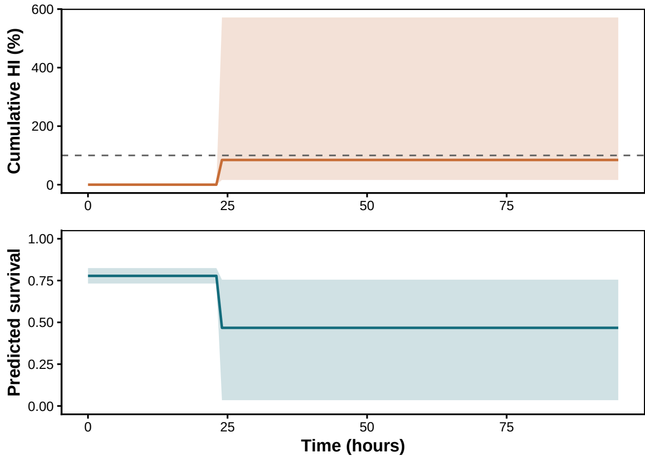
Figure S47: Cumulative heat injury (top) and predicted survival (bottom) under the single-spike trace, no repair . Because the spike sits at the posterior median CT_{max_{1hr}} , ~100% LT50-dose accrues by the end of the spike hour, producing ~50% mortality.
