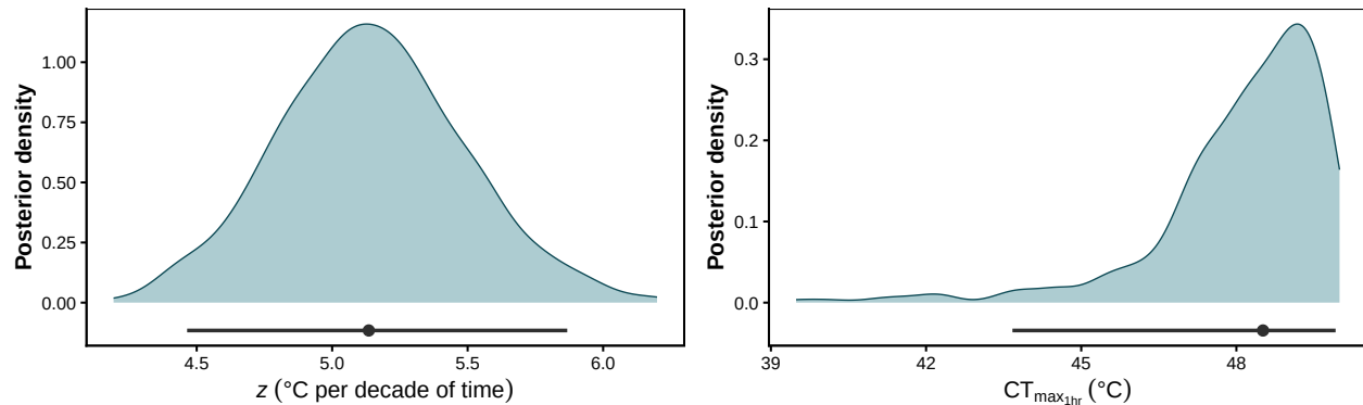
Figure S44: Posterior densities of z (left) and CT_{max1hr} (right) for snow gum leaf PSII function. The horizontal bar below each density is the 95% credible interval; the point marks the posterior median. The \sim 5 °C gap between CT_{max1hr} and T_{crit} is the window between the onset of detectable damage accumulation and the LT50 temperature at 1 h.
