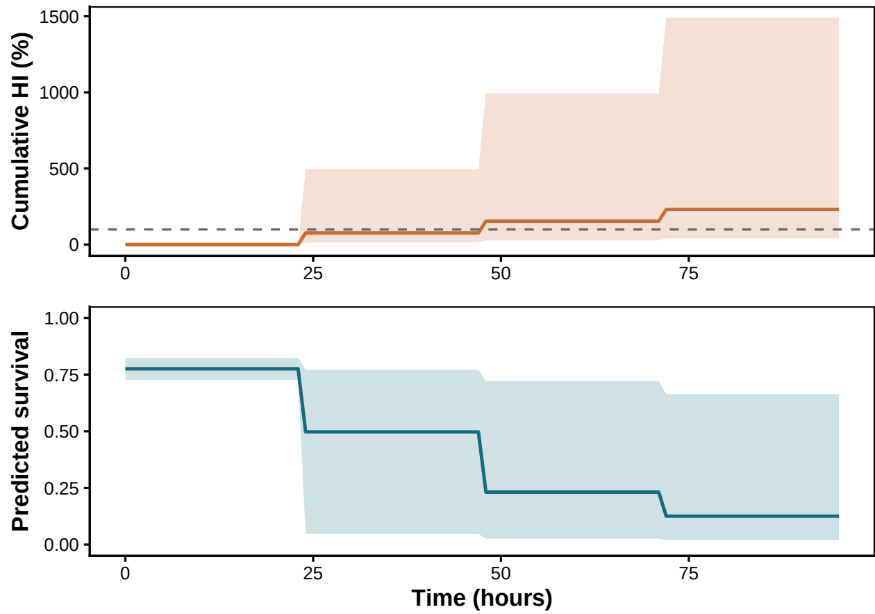
Figure S48: Multi-spike trace, no repair. Three 1-hour spikes at CT_{max_{1hr}} deliver \sim 3 \times \text{LT50-dose} , driving cumulative HI well past 100% and survival to near zero.
