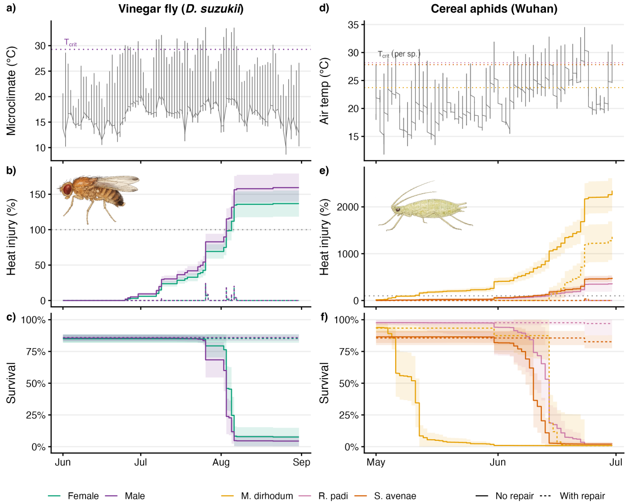
Figure S23: Manuscript Figure 6. Heat-injury accumulation and predicted survival under field temperature trajectories for the vinegar fly ( Drosophila sukuzii , by sex; panels a-c) and three cereal aphids ( Metopolophium dirhodum , Sitobion avenae , Rhopalosiphum padi ; panels d-f). (a, d) the temperature trace — shaded NicheMapR microclimate temperature for the fly (Rennes, France, Jun–Aug 2018; Ørsted et al. 2024 Zenodo record 10821572) and the unmodified hourly air-temperature trace for the aphids (Wuhan, May–June 2016; Li et al. 2023, Open-Meteo ERA5) — with the relative-threshold T_{crit} (dotted; per species for the aphids). (b, e) cumulative heat injury (100% = one LT_{50} dose, dotted grey) and (c, f) predicted survival, each with and without damage repair (line type). Fly panels are coloured by sex, aphid panels by species. Bands are \pm 1 SE across posterior draws. Predicted survival begins at each group’s fitted upper asymptote rather than at 100% (the vinegar-fly 4PL estimates a maximum survival of 85%, up < 1 ). Repair uses an illustrative Sharpe–Schoolfield kernel with an Arrhenius (uninhibited) rate scale r_{ref} = 0.03 LT_{50} -dose h^{-1} ; it is not empirically fitted.
