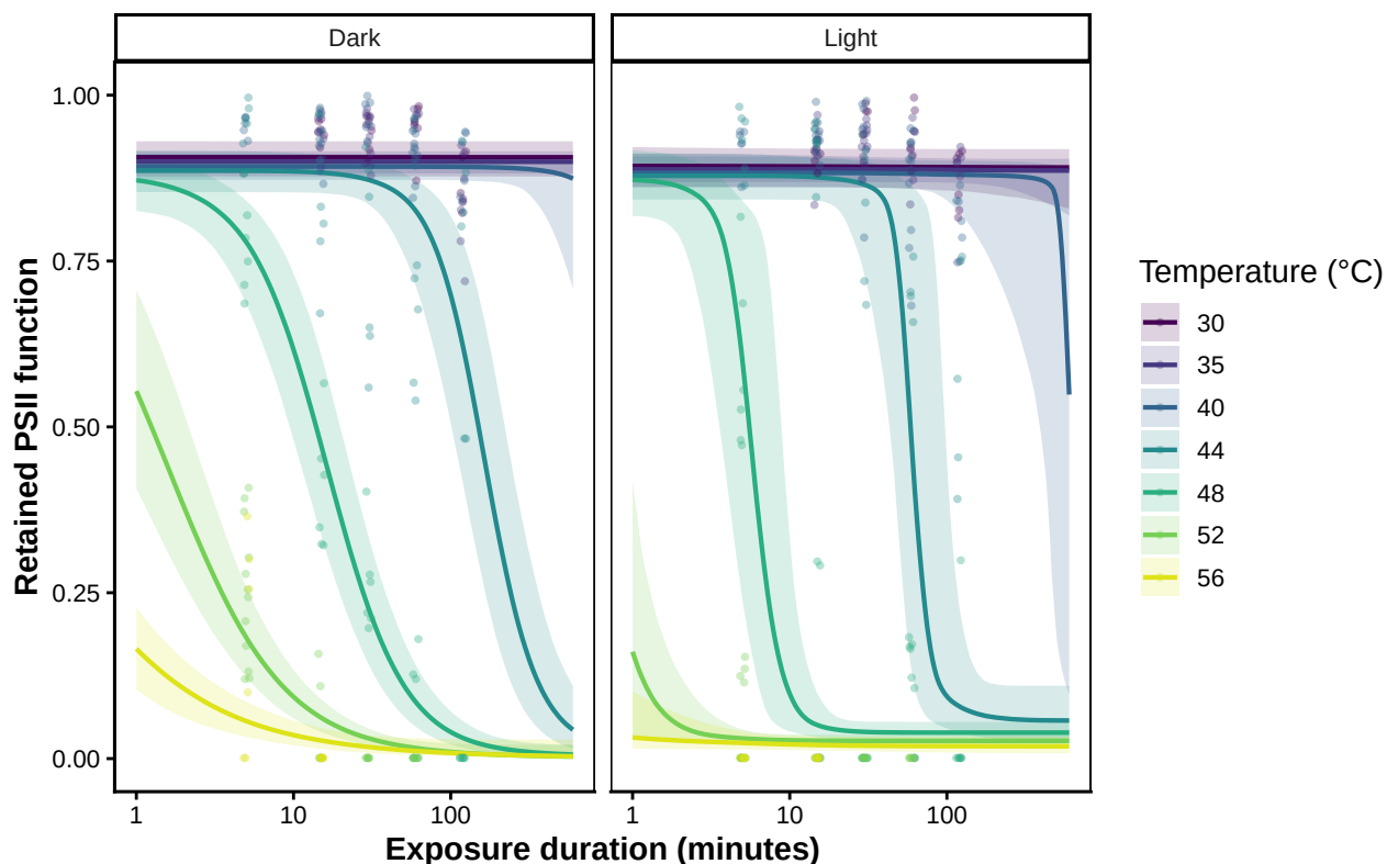
Figure S14: Fitted retained-PSII-function surfaces for snow gum under dark and light post-heat recovery (posterior median and 95% credible band), with observed per-replicate proportions overlaid. The light-recovery curves cross the midpoint at shorter durations, the visual signature of the lower CT_{max} .
