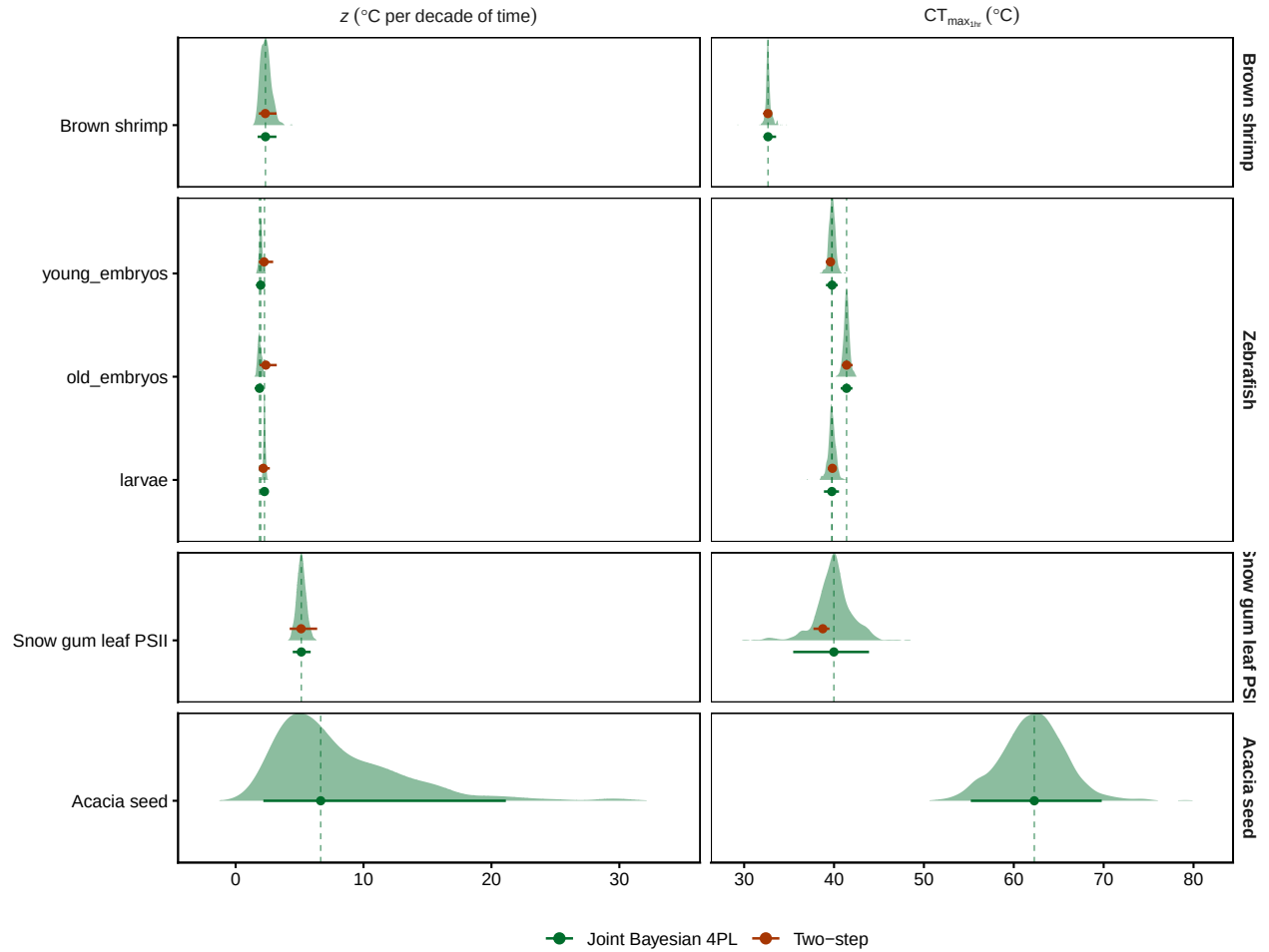
Figure S57: Manuscript Figure 4. Posterior densities of z (left column) and CT_{max1hr} (right column) from the joint Bayesian 4PL fits (green ridges, #006d2c) for the four case studies (rows). The 4PL posterior median and 95% credible interval are overlaid as a green pointrange. The classical two-stage point estimate (beta-binomial Stage 1 for the brown shrimp and zebrafish counts, beta Stage 1 for the snow gum leaf PSII proportions) is shown for comparison as an orange pointrange (median + 95% CI, #a63603); the Acacia seed has no two-stage estimate because its sparse design yields a valid Stage-1 LT50 at too few temperatures. Dashed vertical lines mark the 4PL posterior median for each entity. The zebrafish panel splits into three ridges, one per life stage. Panels use free x-axes; the seed z posterior is wide, reflecting an assay design whose durations do not bracket the LT50 at most temperatures.
