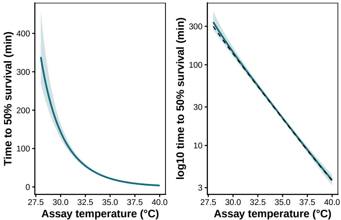
Figure S6: Posterior \text{LT50}(T) curve (median + 95% CrI, blue) recovered by derive_tdt_curve() from the T -varying fit, with the analytical truth overlaid (dashed black). The curve is visibly bent rather than straight in T , and the posterior tracks the truth.
