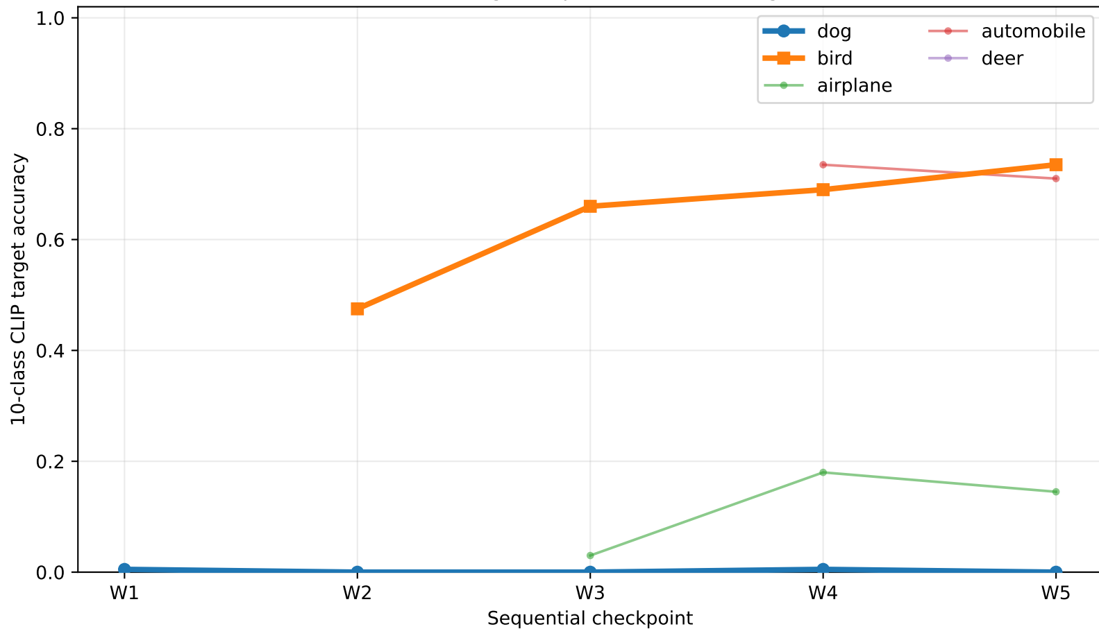
Clean-chain target trajectories (200 images/cell)
