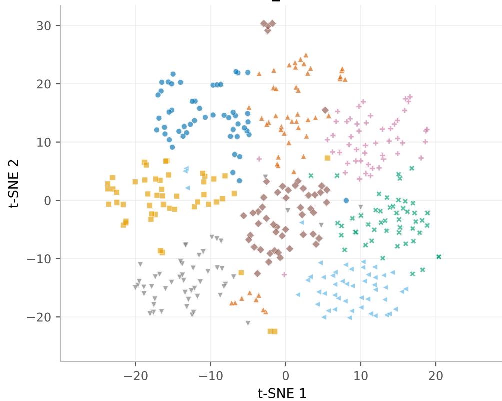
random_state = 0
