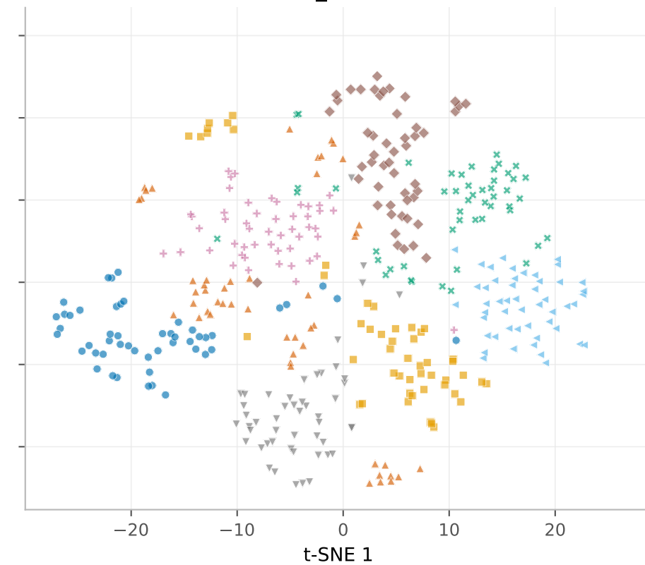
random_state = 42
