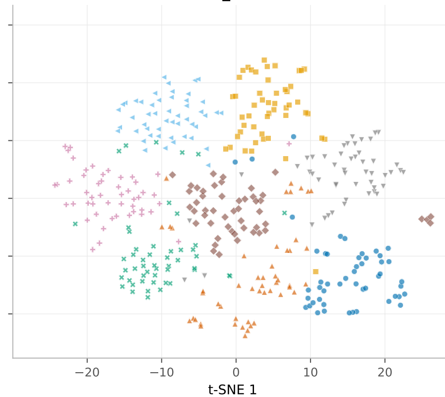
random_state = 1
