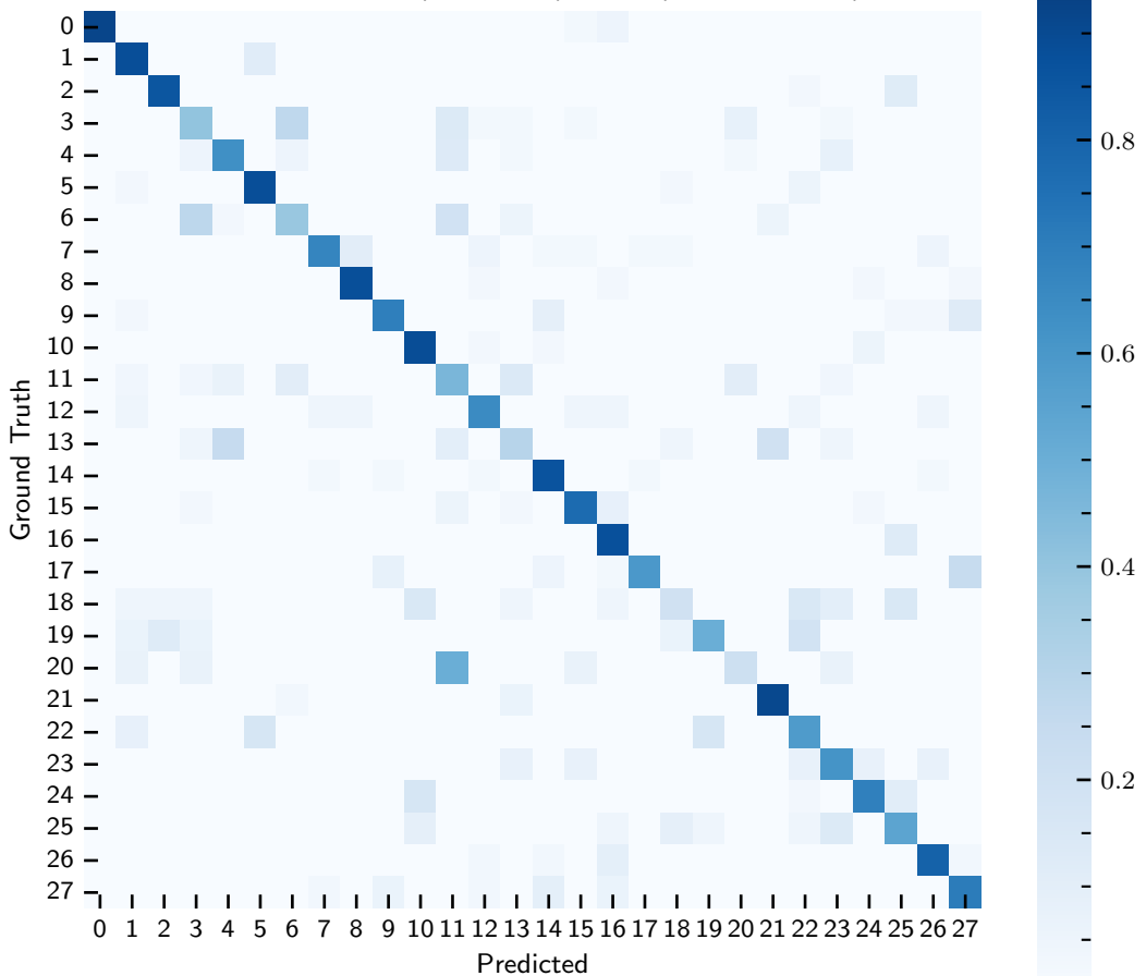
Confusion Matrix (normalized) — B0 (Baseline Fusion)
