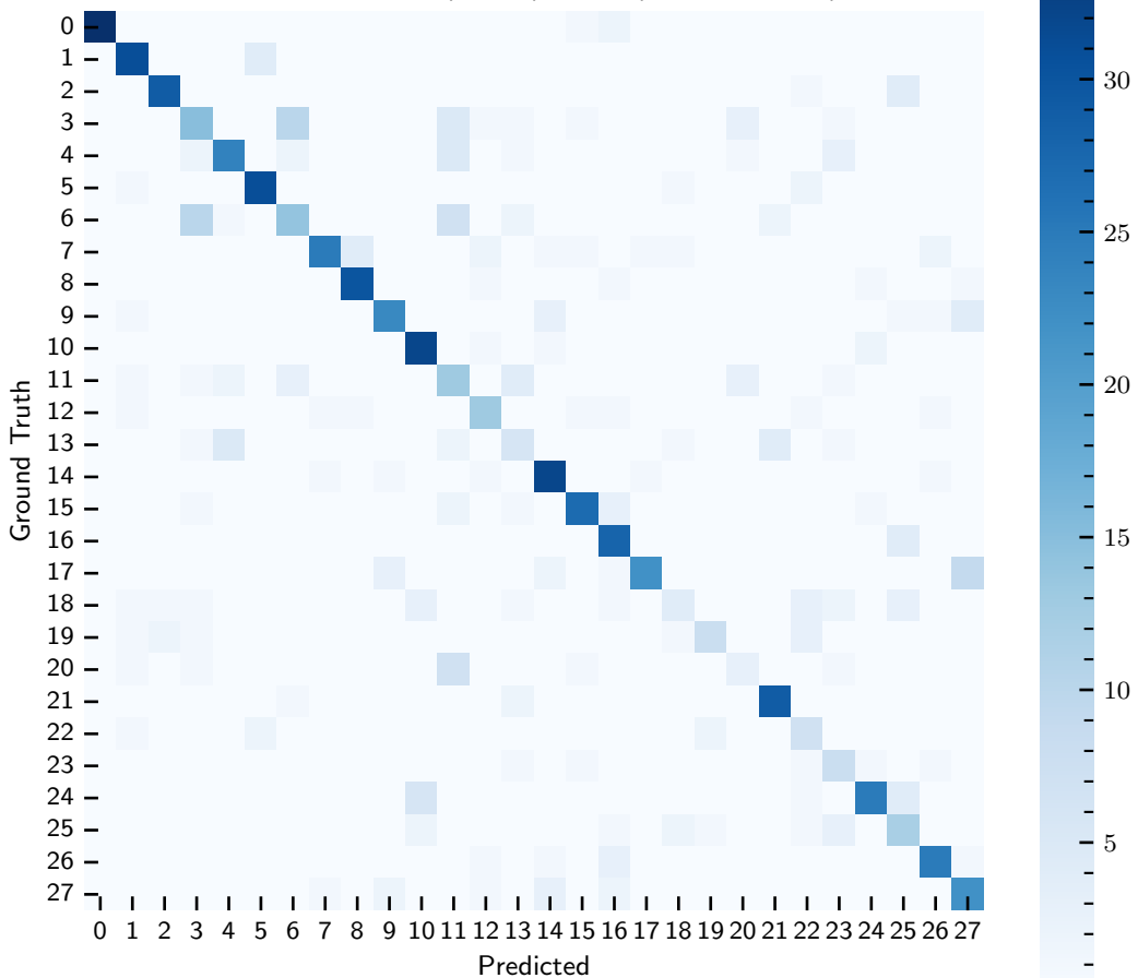
Confusion Matrix (counts) — B0 (Baseline Fusion)
