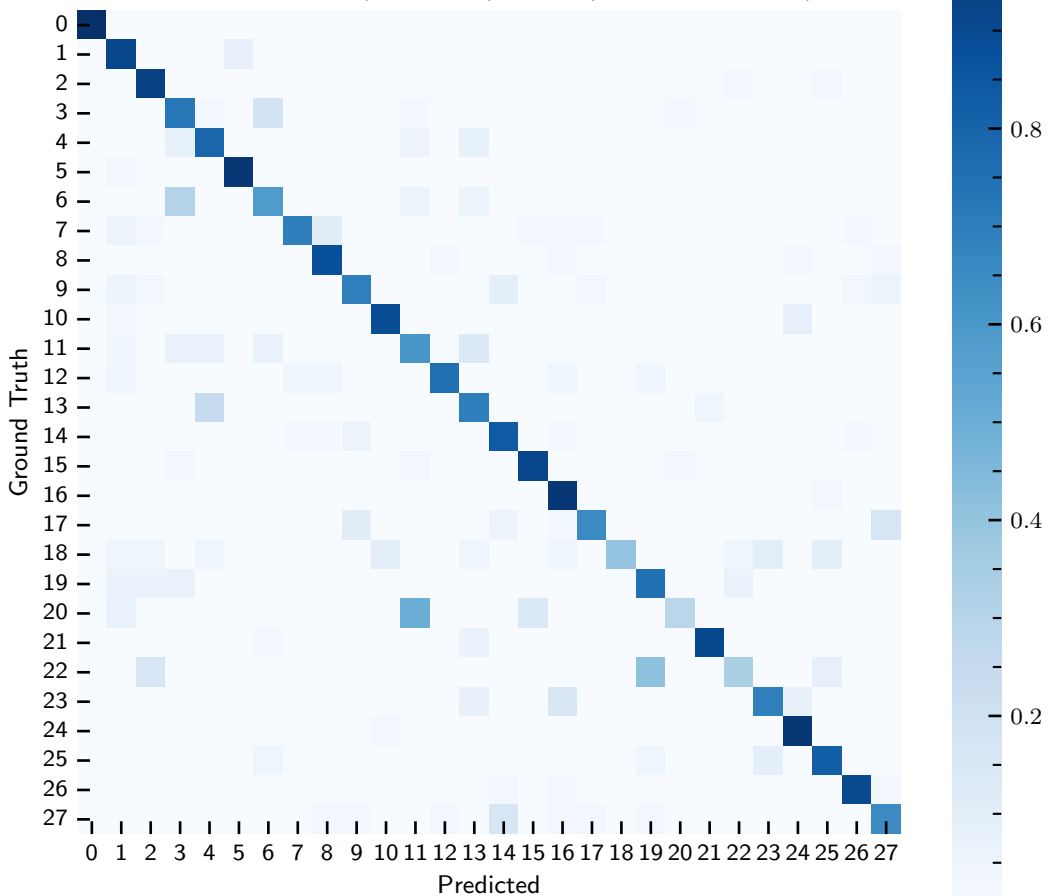
Confusion Matrix (normalized) — M1 (Attention + Hedge)
