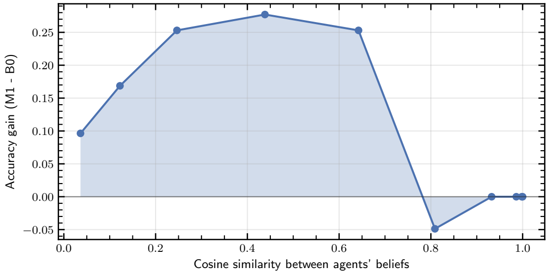
Fusion Gain vs. Disagreement (cosine)
