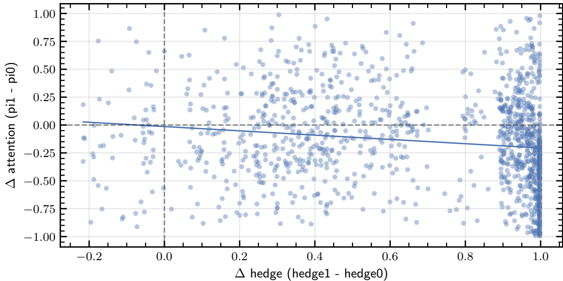
Alignment of Hedge and Attention
